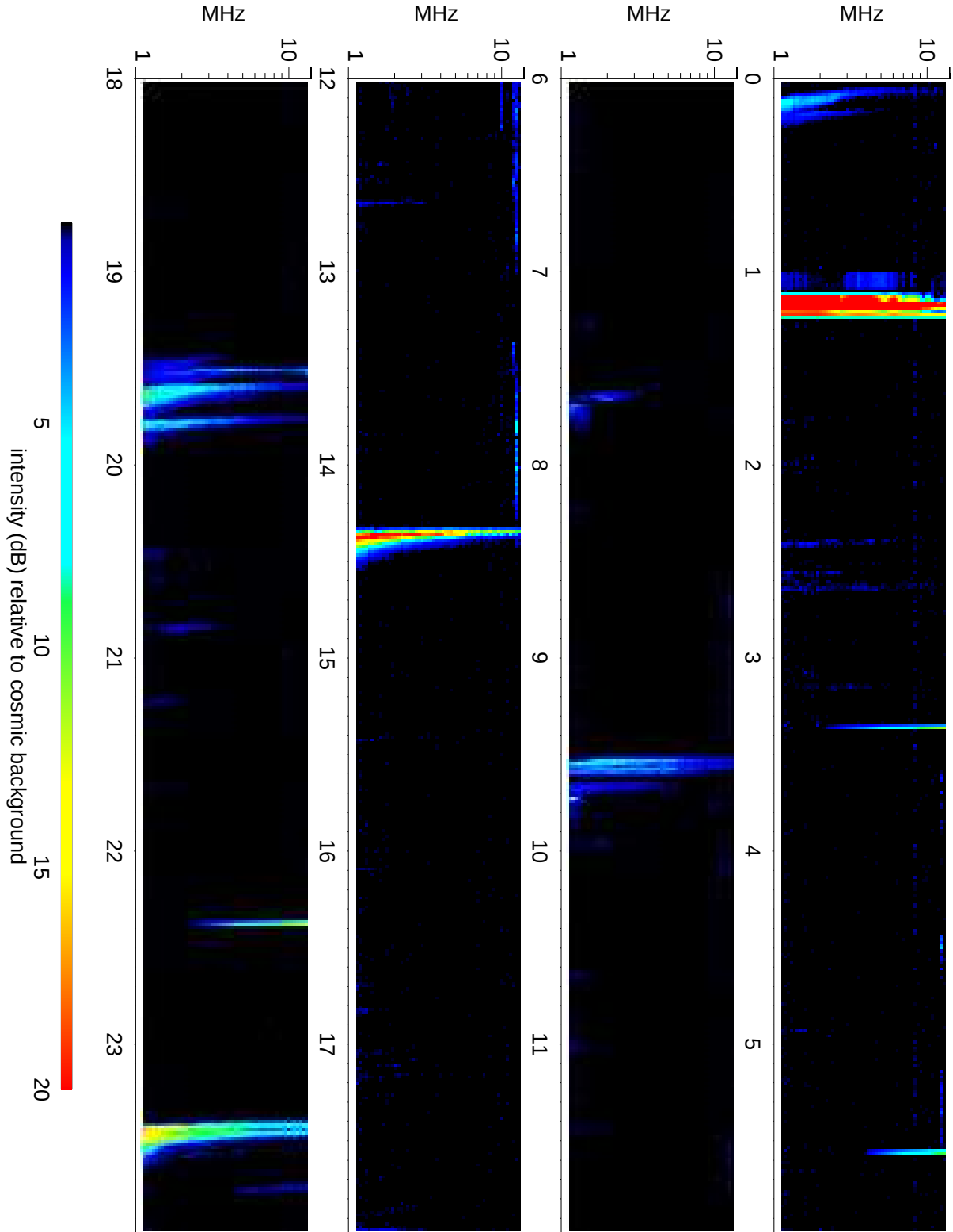
Wind Waves RAD2 receiver: 2011/03/03
