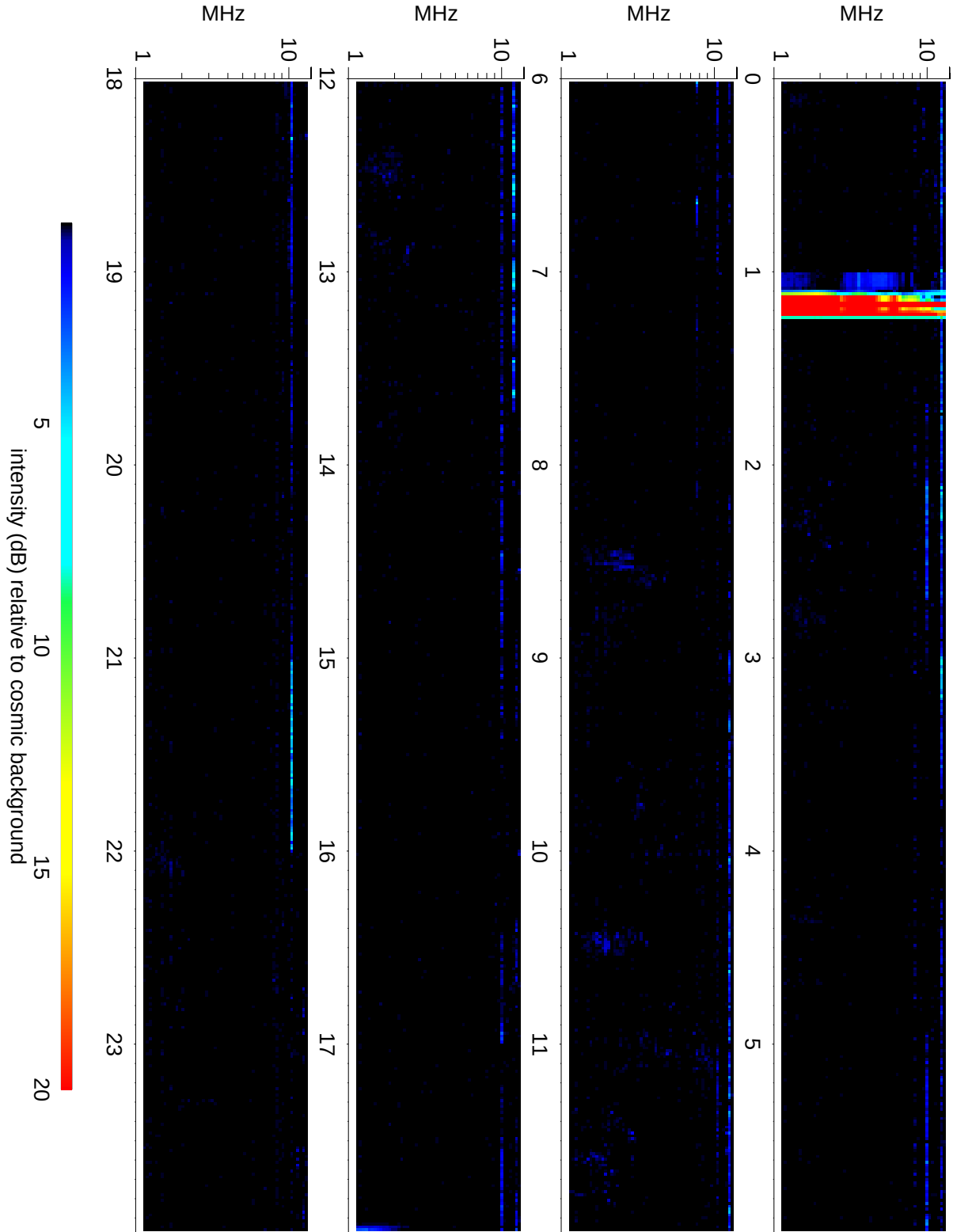
Wind Waves RAD2 receiver: 2011/01/10
