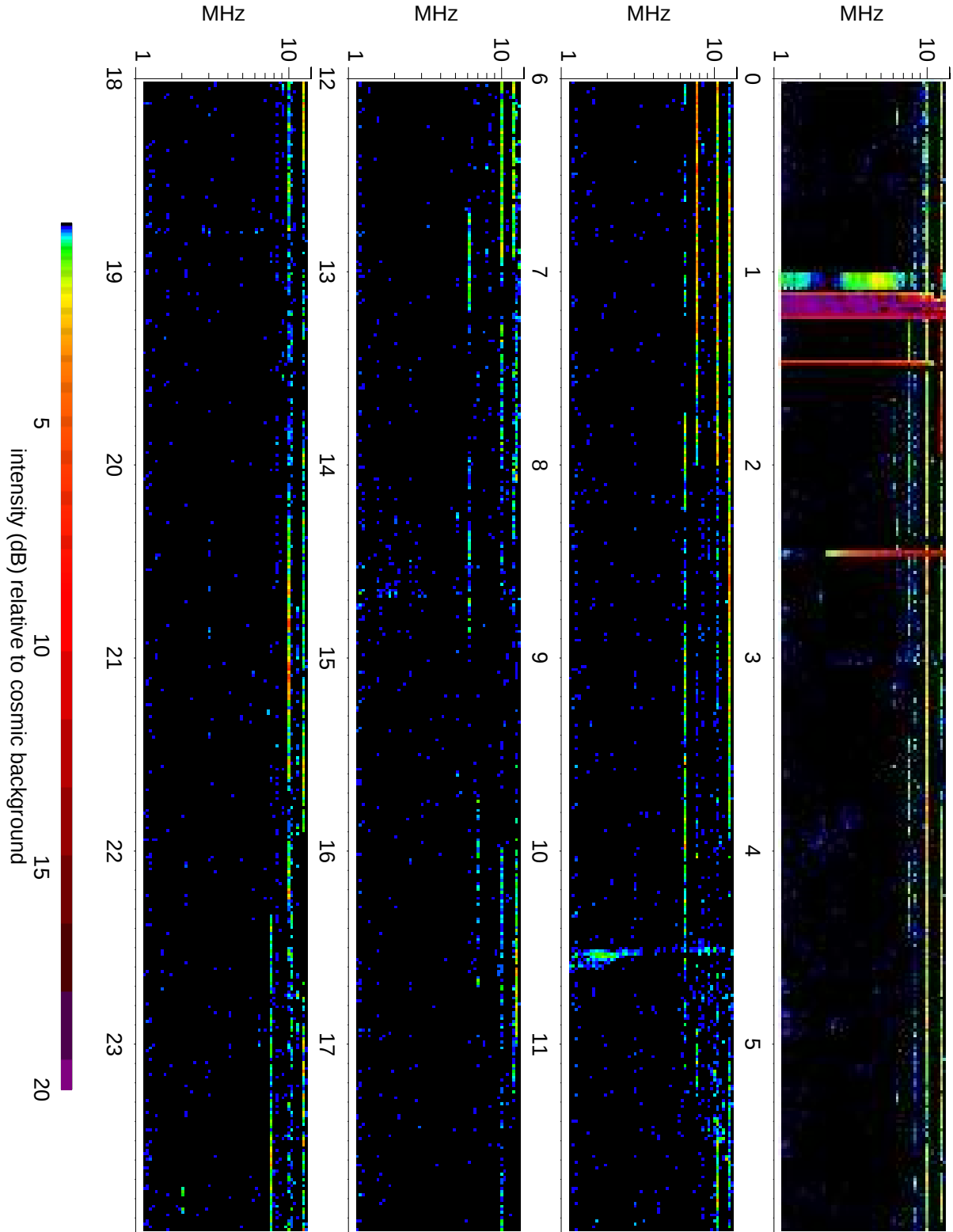
Wind Waves RAD2 receiver: 2010/06/17
