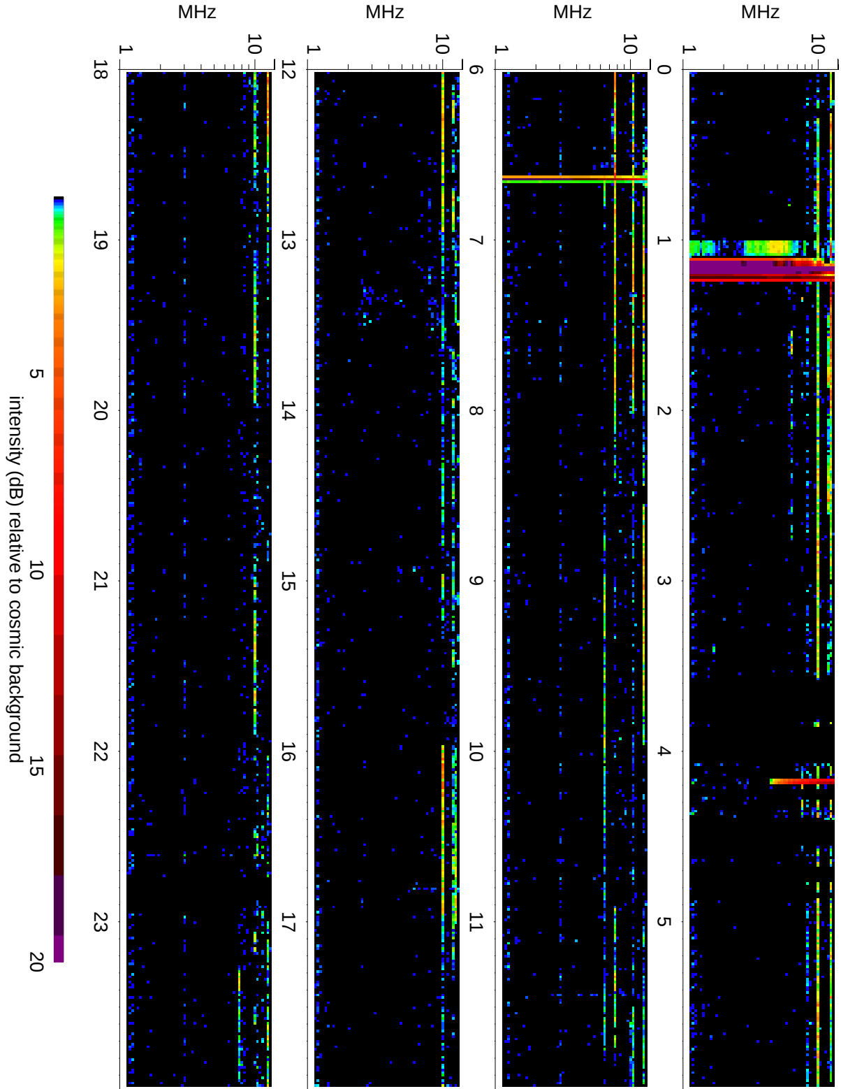
Wind Waves RAD2 receiver: 2010/06/01
