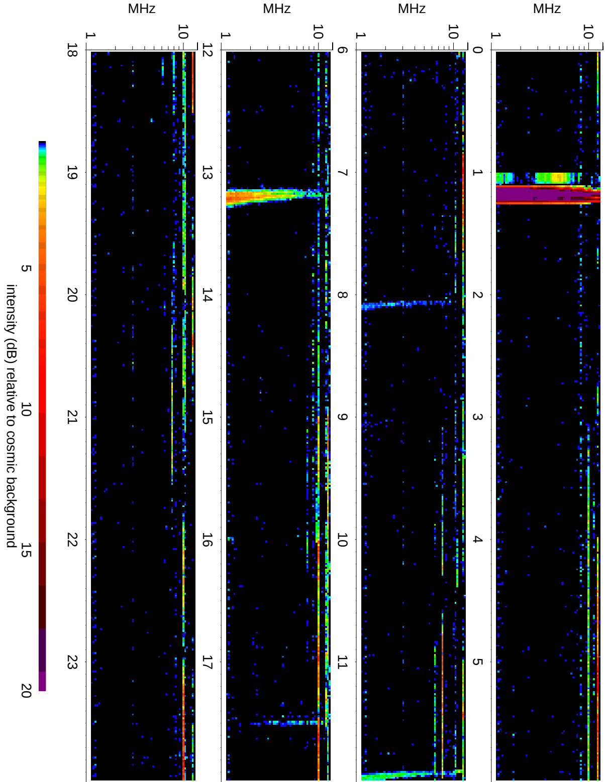
Wind Waves RAD2 receiver: 2010/04/06
