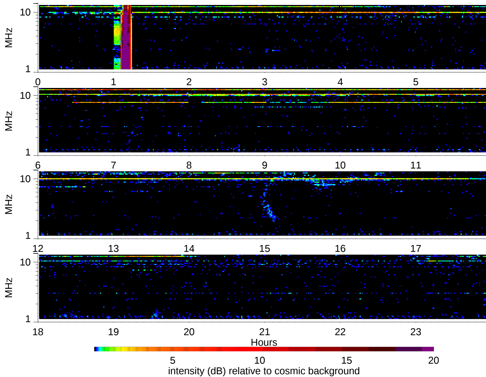
Wind Waves RAD2 receiver: 2008/9/14
