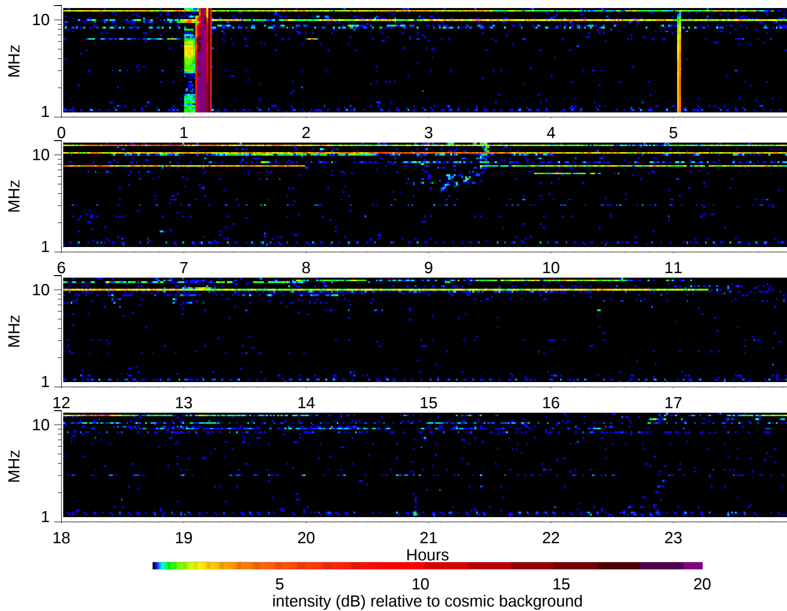
Wind Waves RAD2 receiver: 2008/9/8
