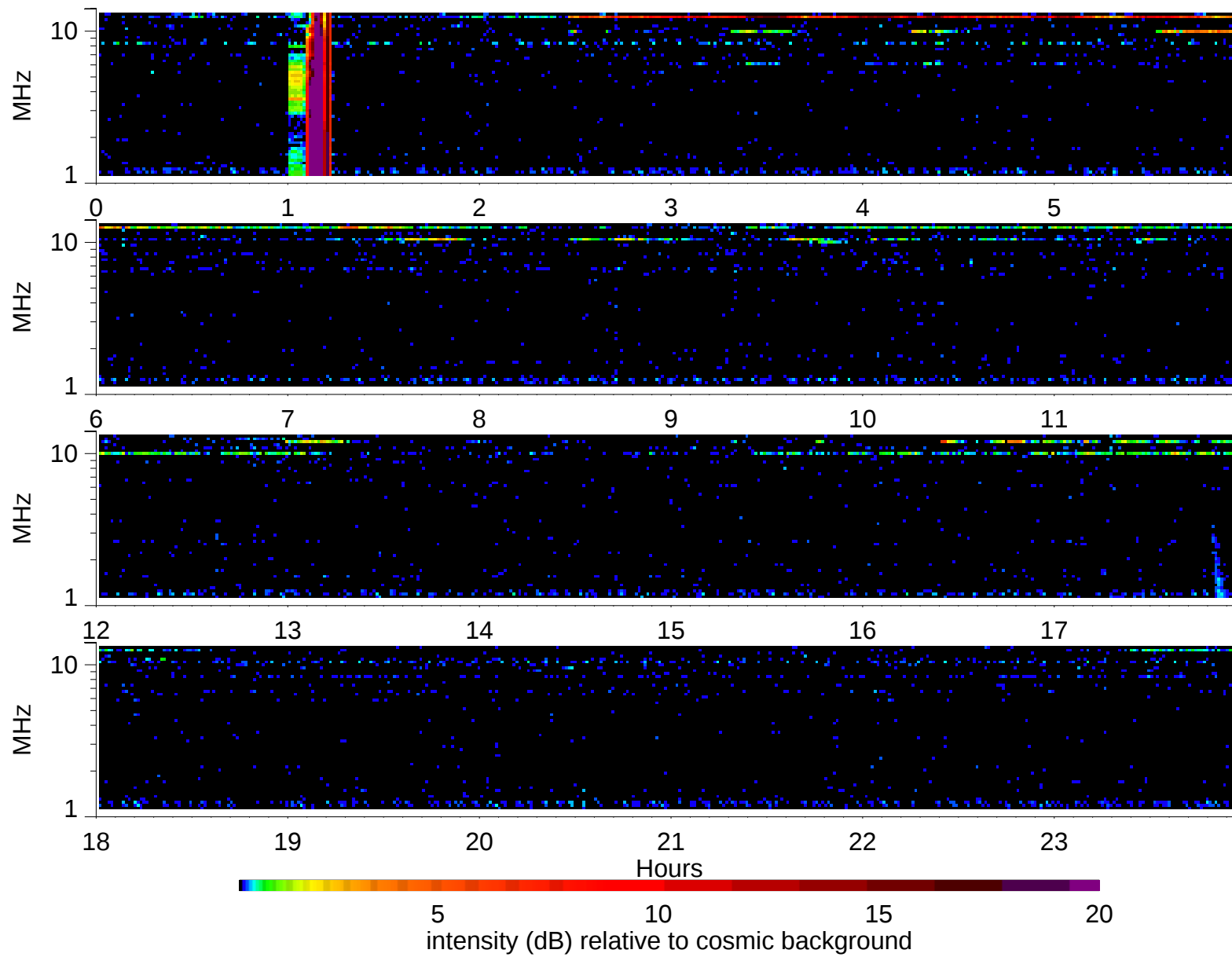
Wind Waves RAD2 receiver: 2007/12/14
