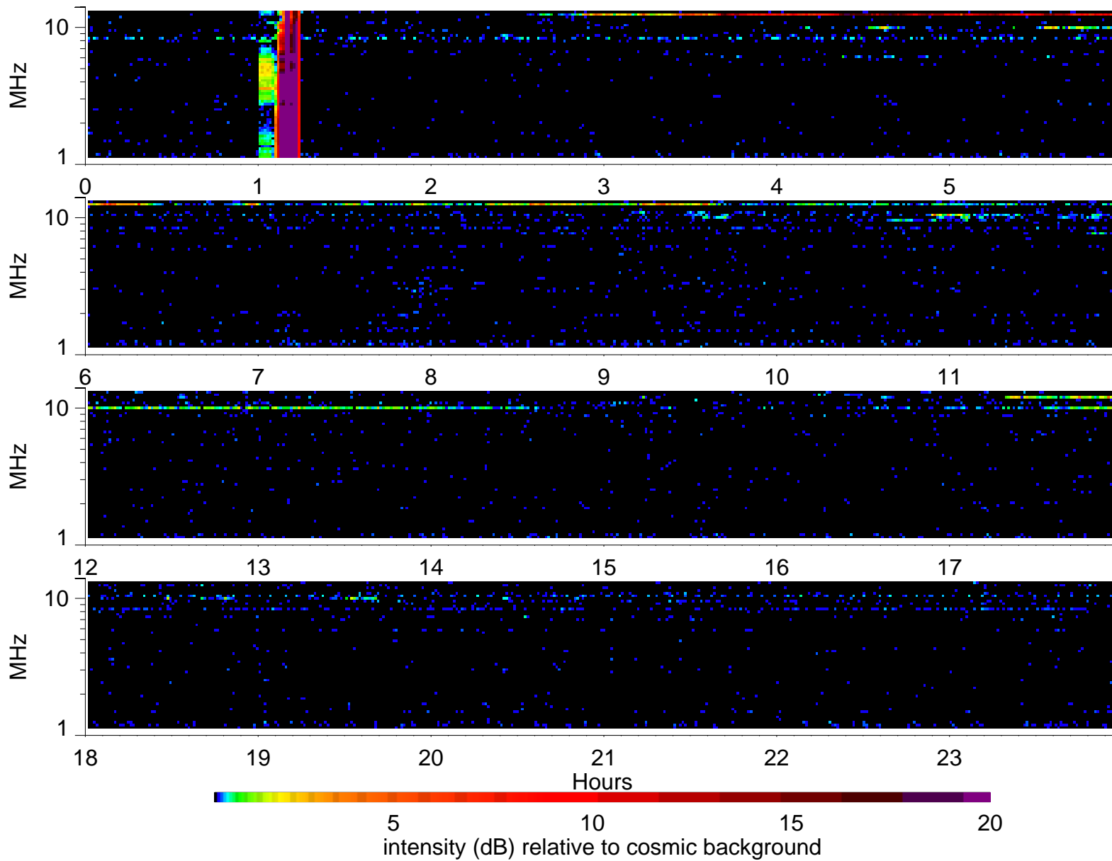
Wind Waves RAD2 receiver: 2007/11/18
