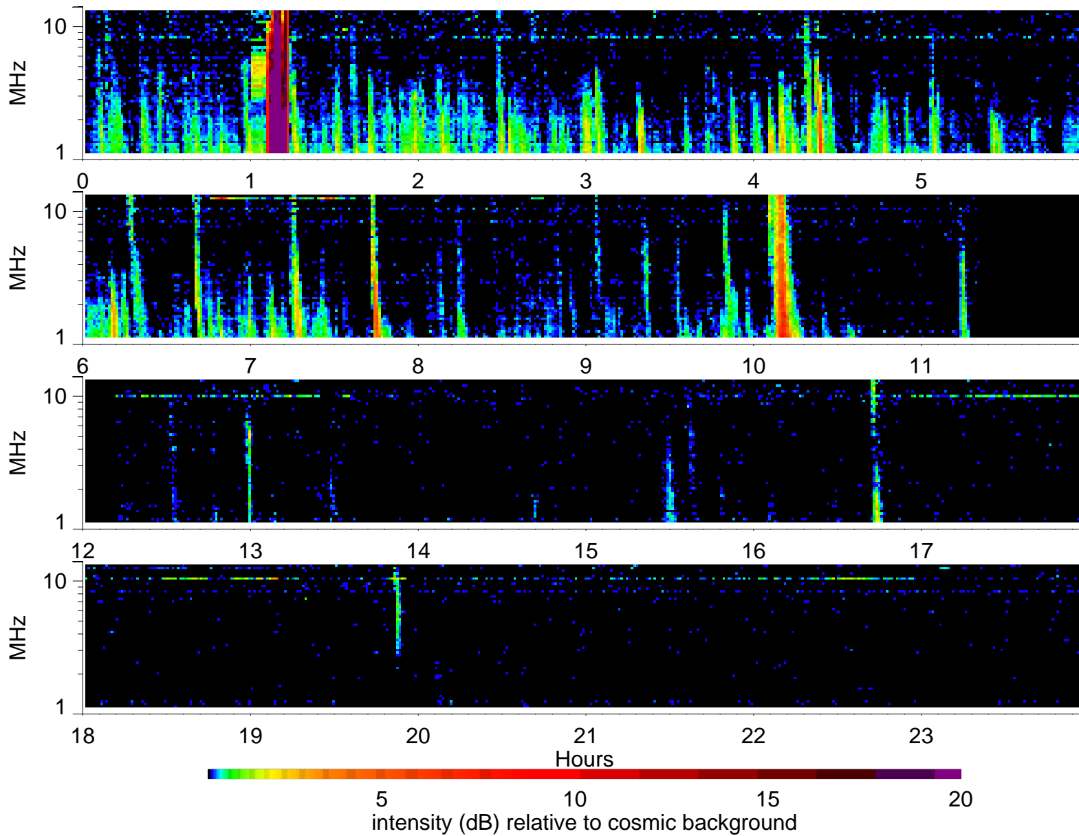
Wind Waves RAD2 receiver: 2006/11/18
