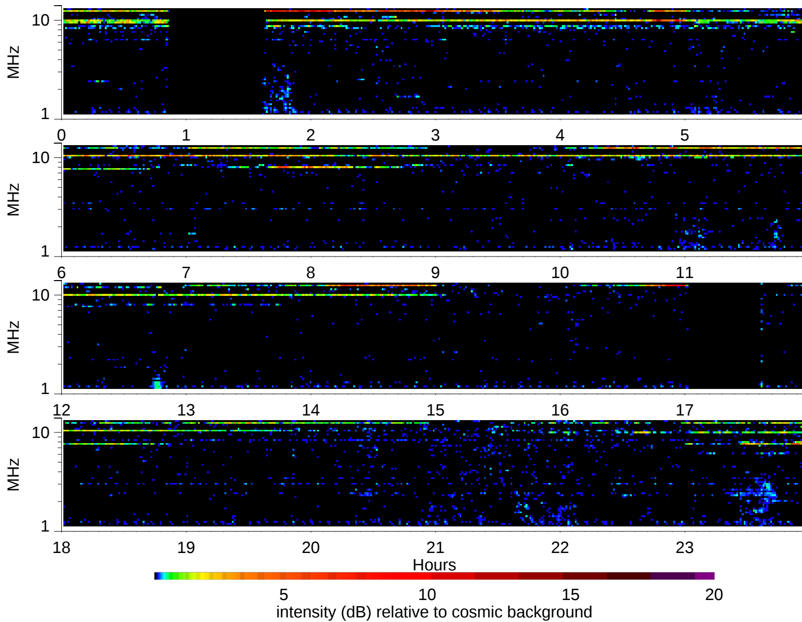
Wind Waves RAD2 receiver: 2006/9/5
