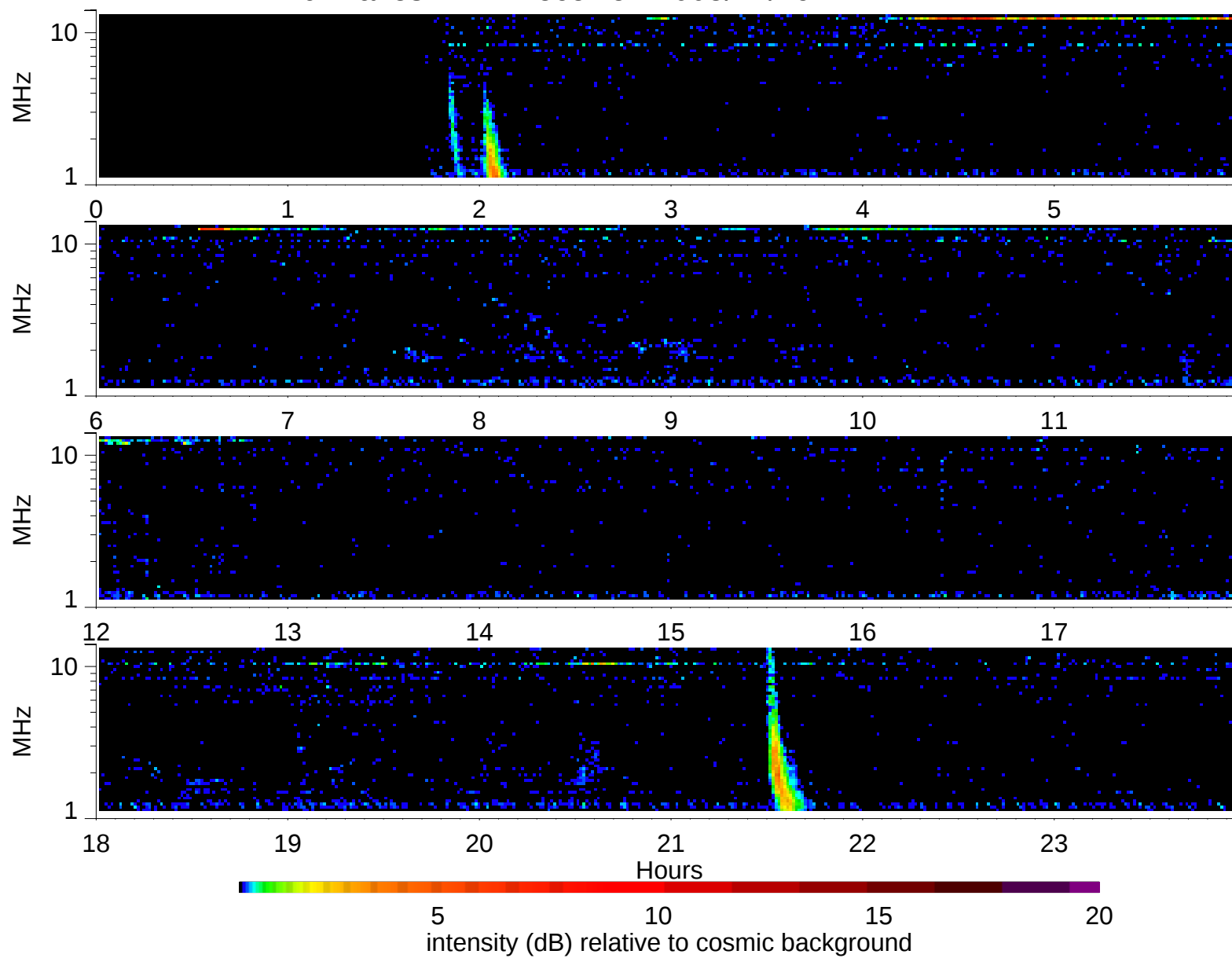
Wind Waves RAD2 receiver: 2005/12/19
