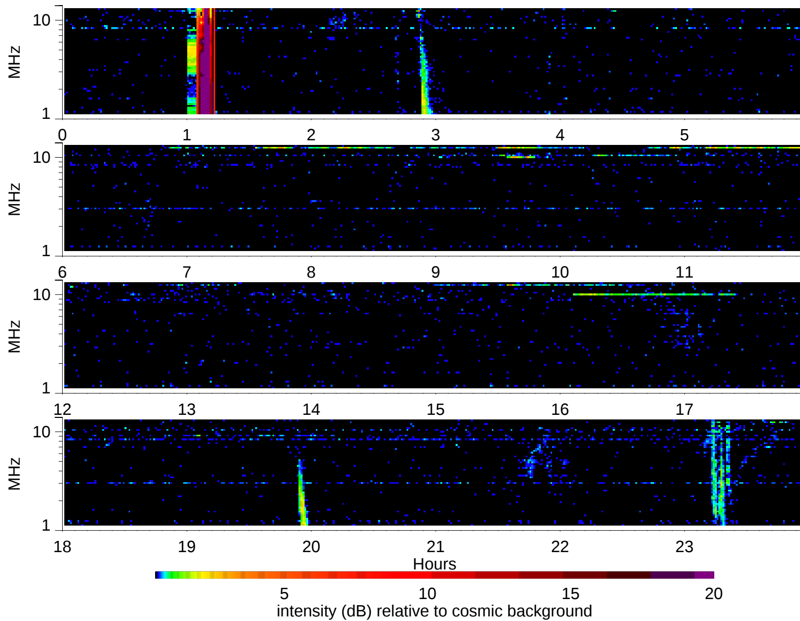
Wind Waves RAD2 receiver: 2005/10/9
