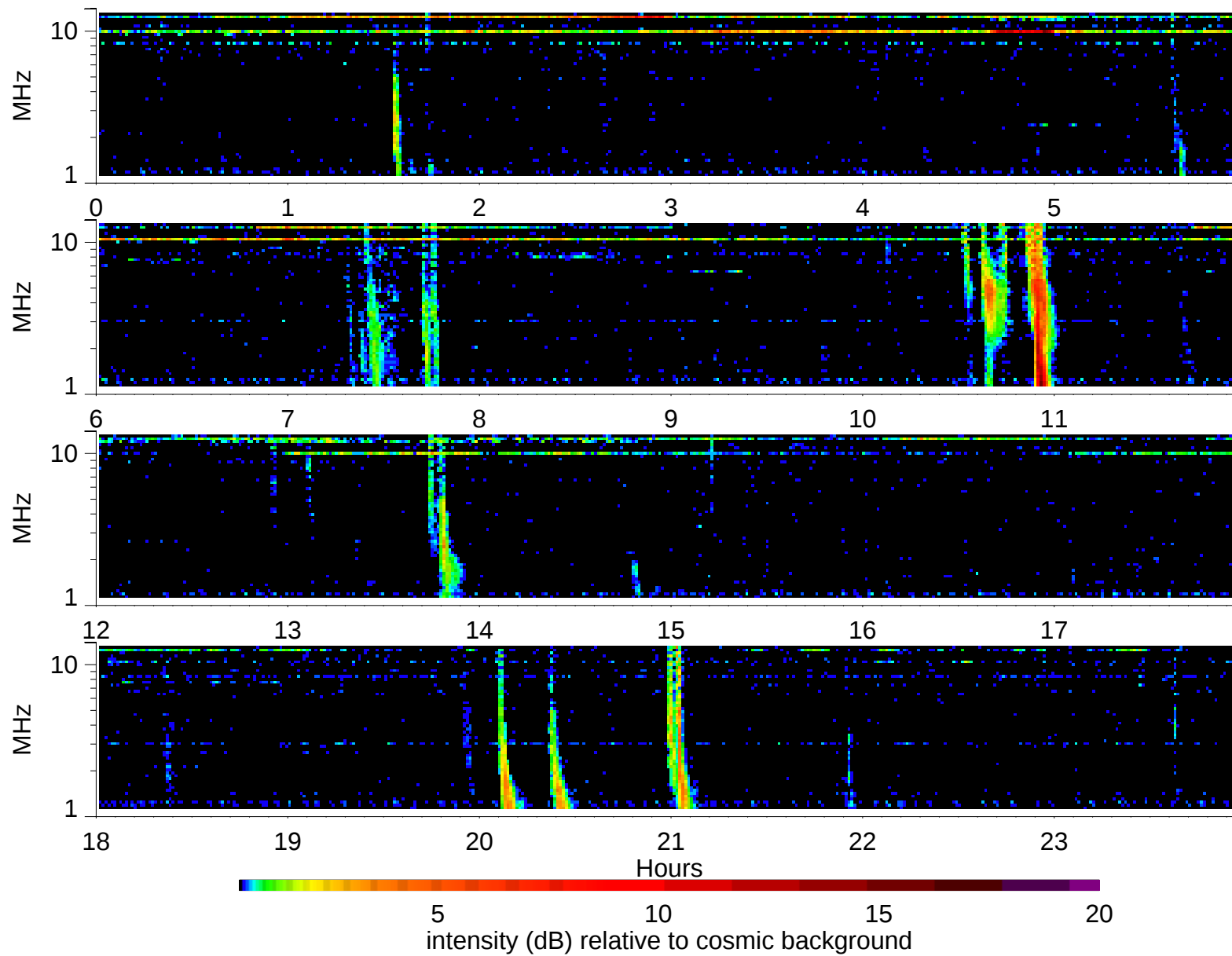
Wind Waves RAD2 receiver: 2005/8/5
