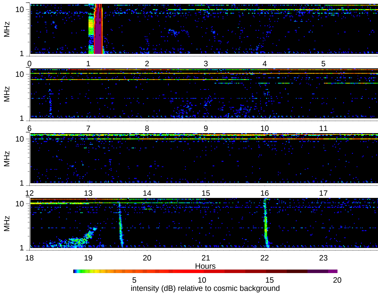
Wind Waves RAD2 receiver: 2005/5/22
