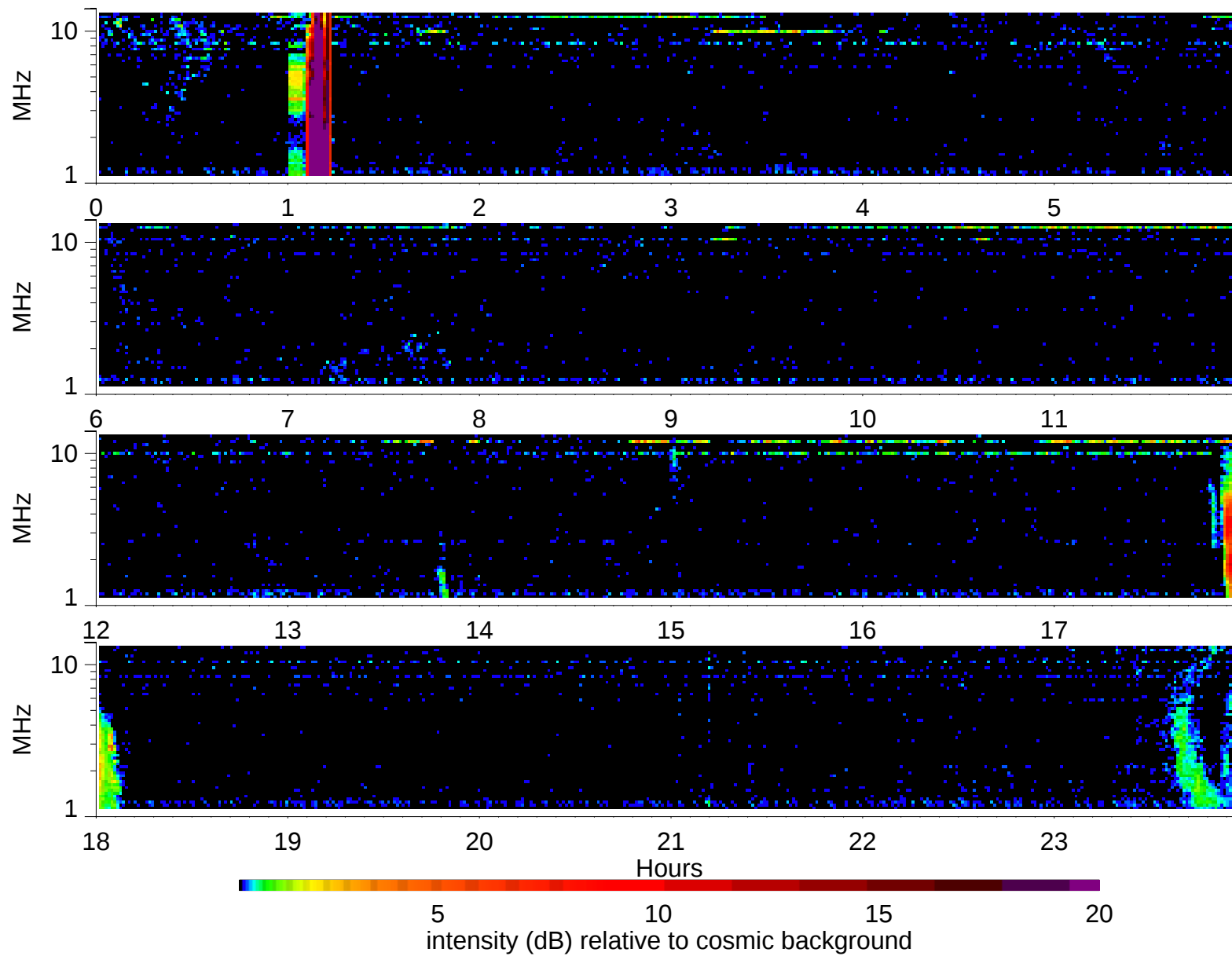
Wind Waves RAD2 receiver: 2005/2/5
