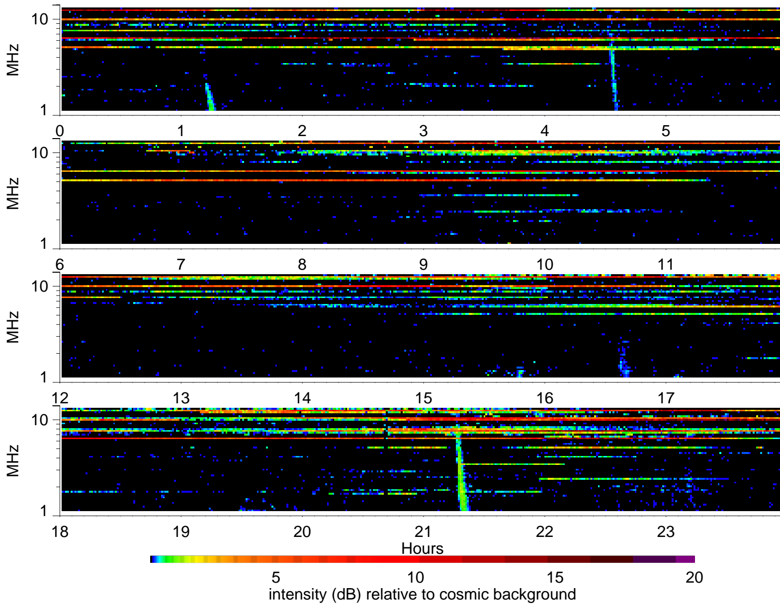
Wind Waves RAD2 receiver: 2004/4/28
