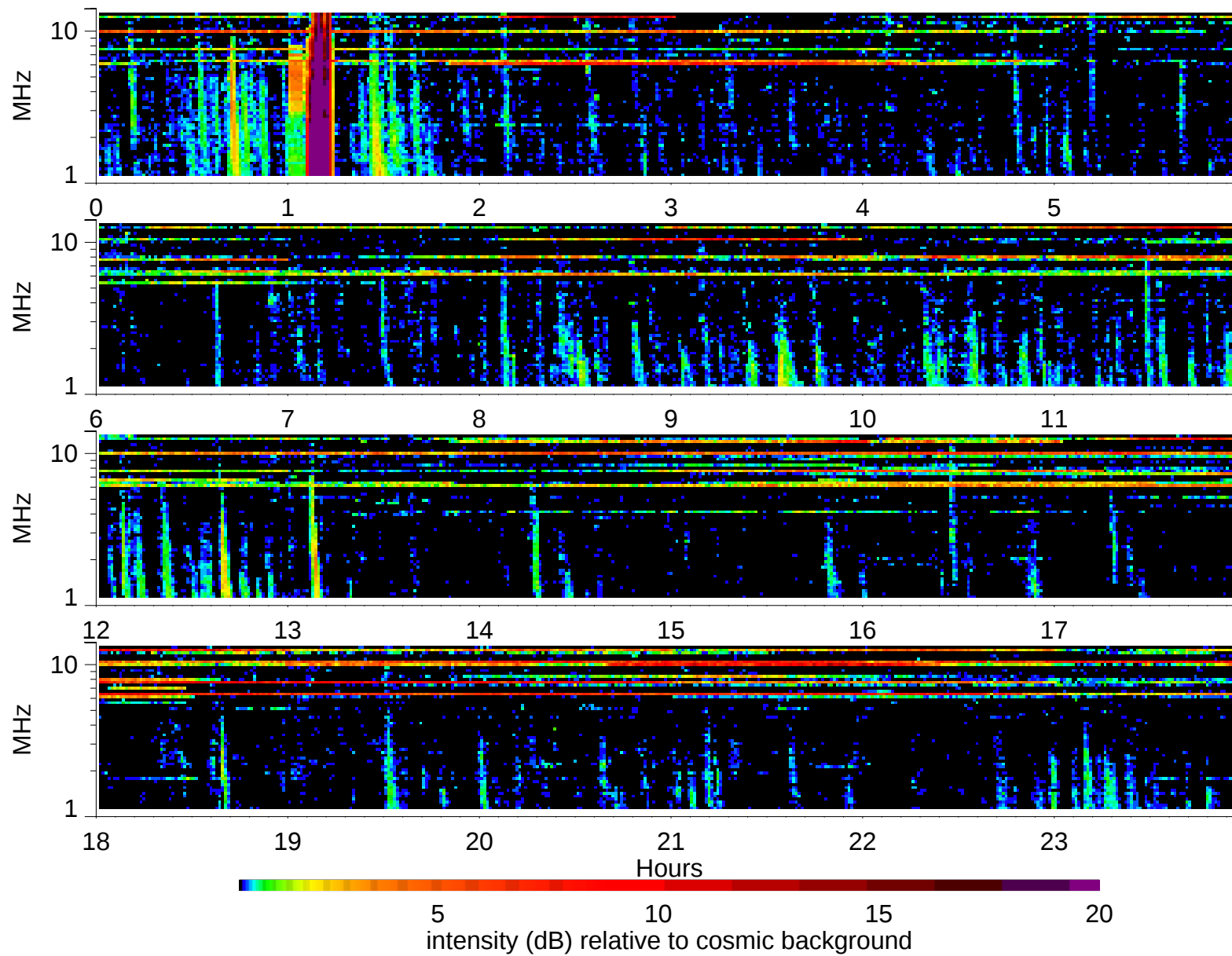
Wind Waves RAD2 receiver: 2003/12/26
