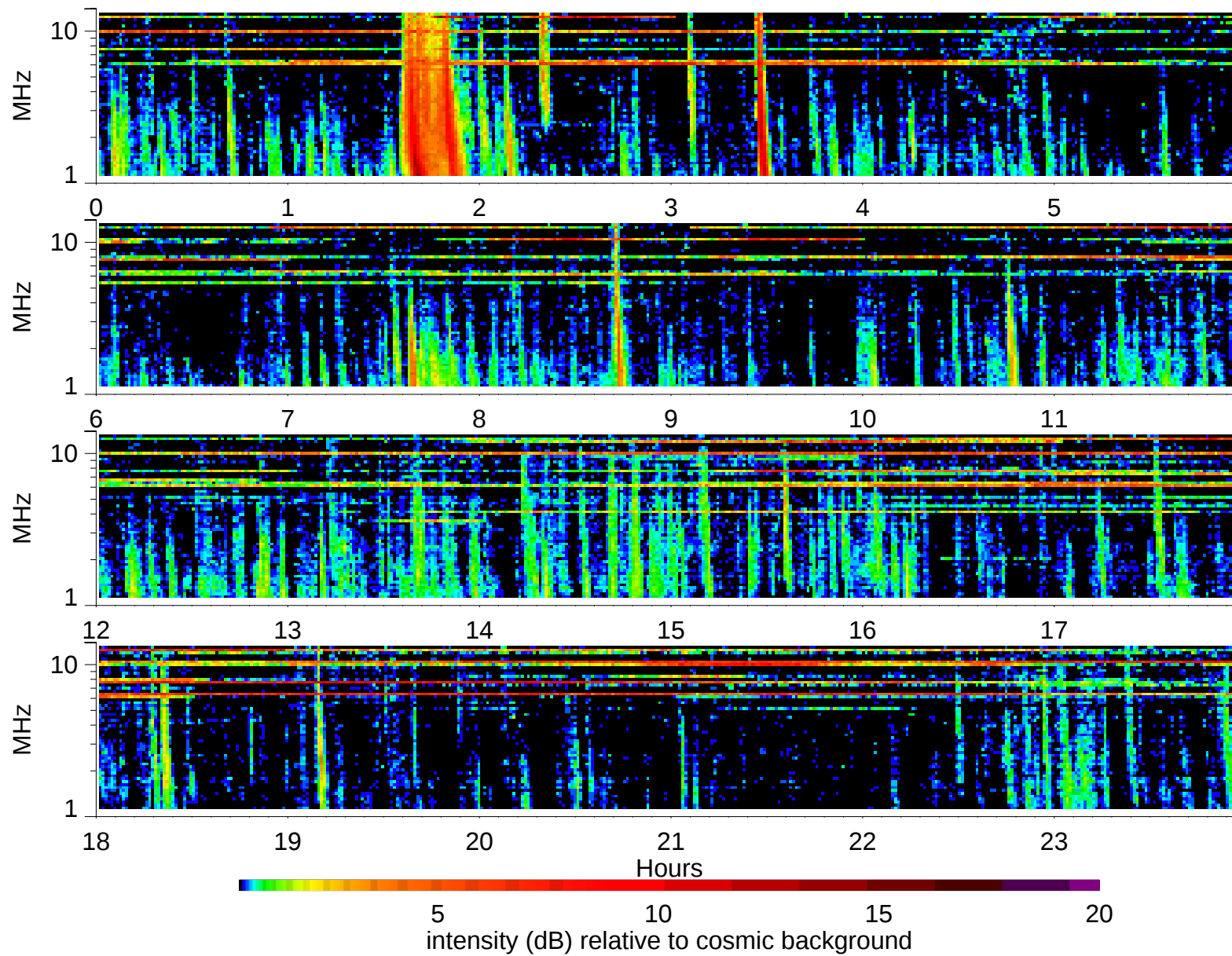
Wind Waves RAD2 receiver: 2003/12/25
