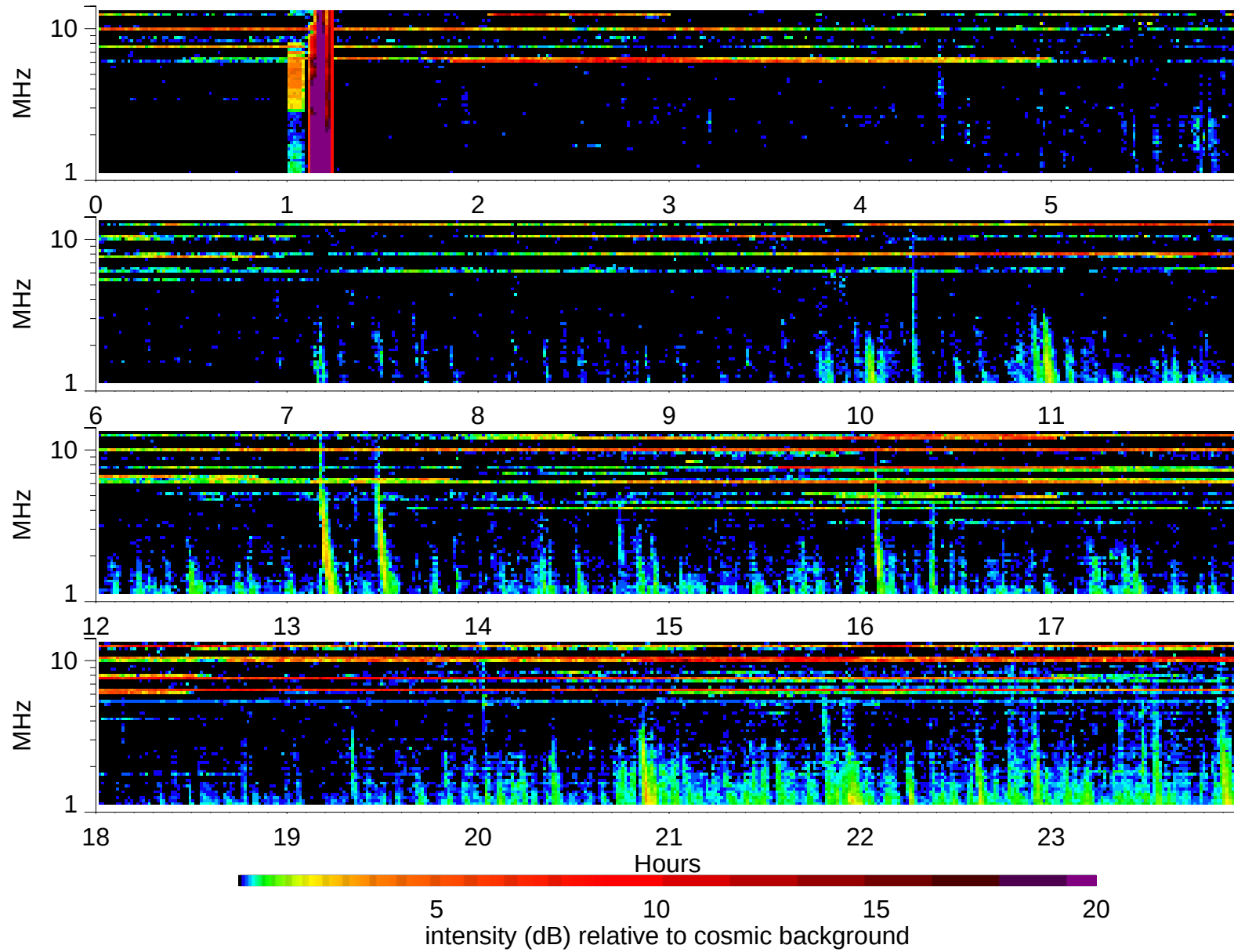
Wind Waves RAD2 receiver: 2003/12/22
