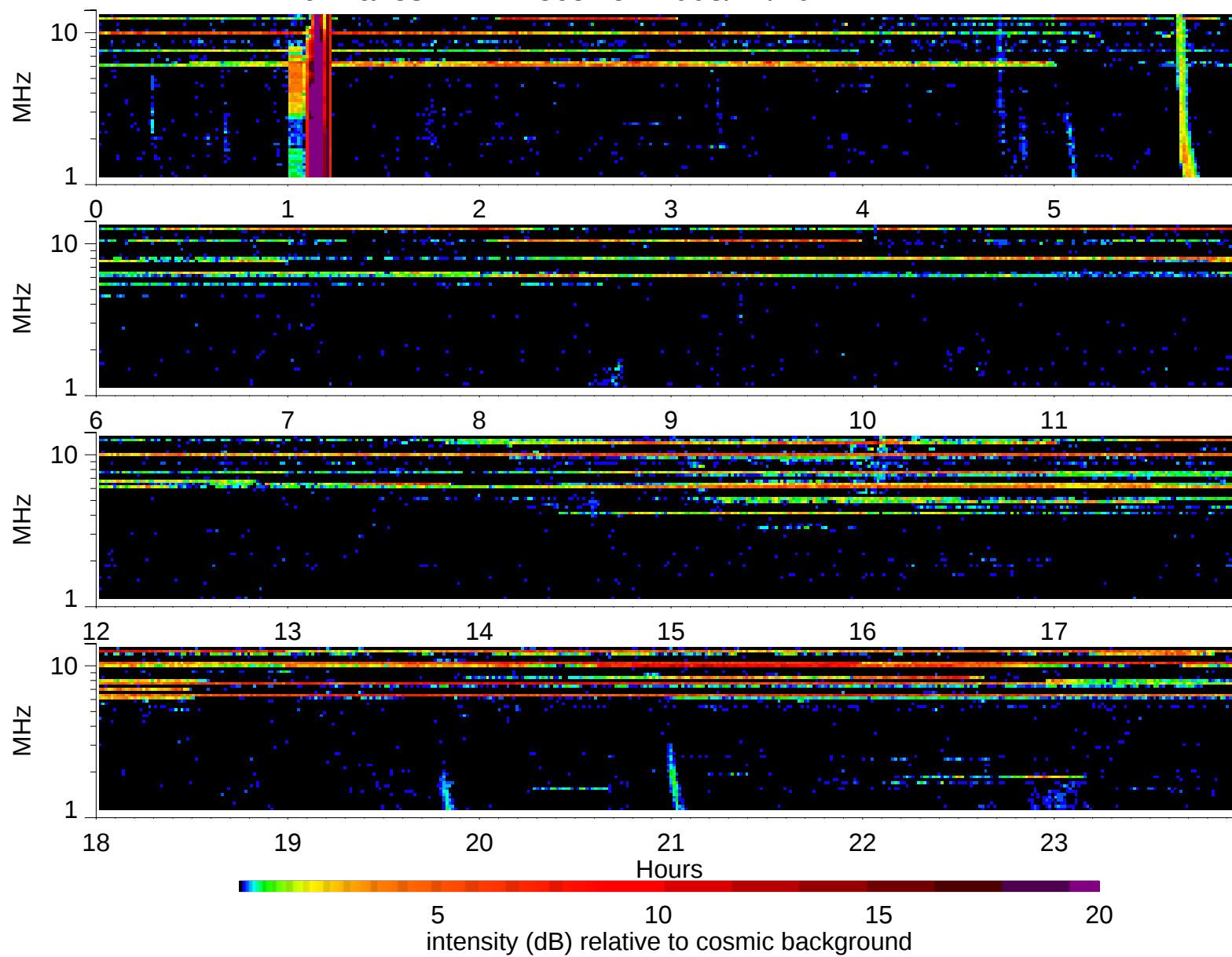
Wind Waves RAD2 receiver: 2003/12/20
