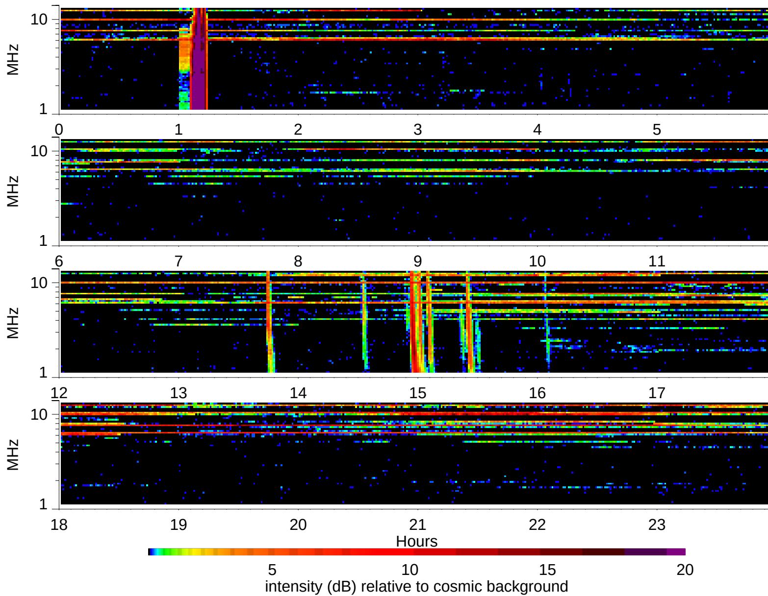
Wind Waves RAD2 receiver: 2003/12/10
