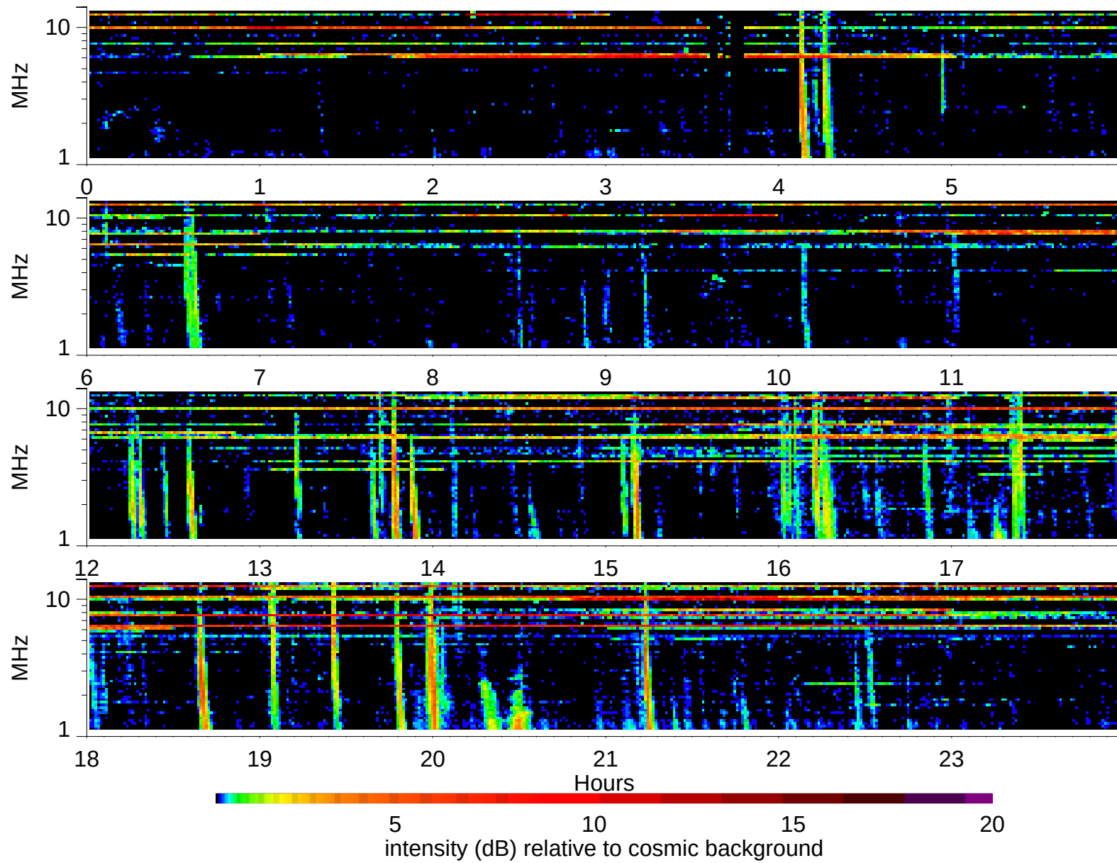
Wind Waves RAD2 receiver: 2003/12/3
