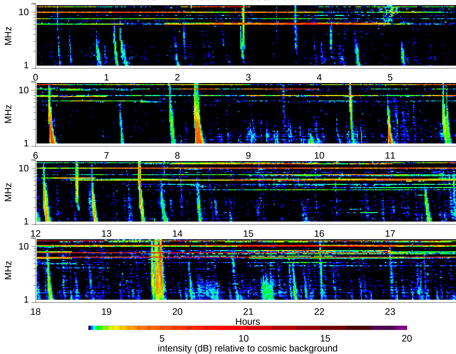
Wind Waves RAD2 receiver: 2003/12/1
