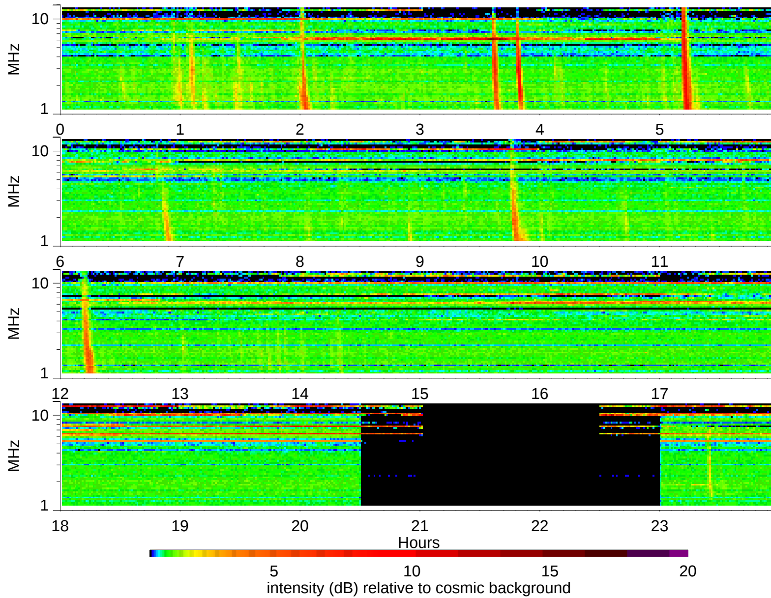
Wind Waves RAD2 receiver: 2003/11/27
