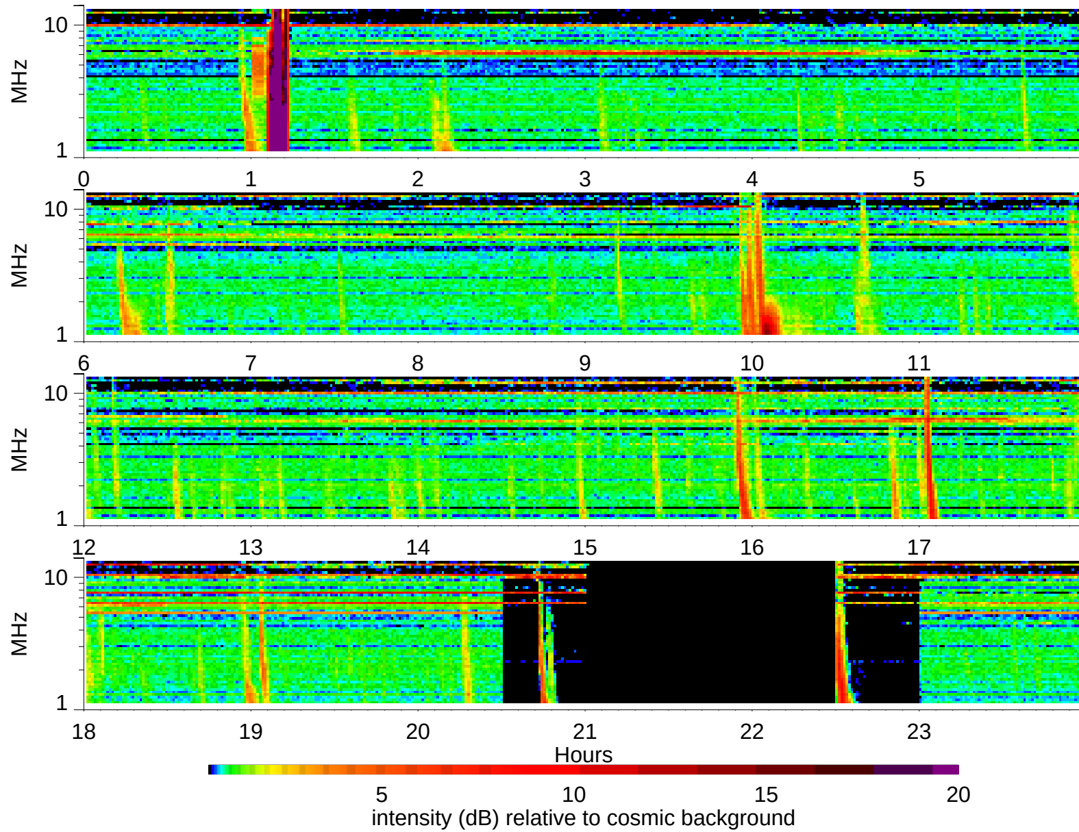
Wind Waves RAD2 receiver: 2003/11/26
