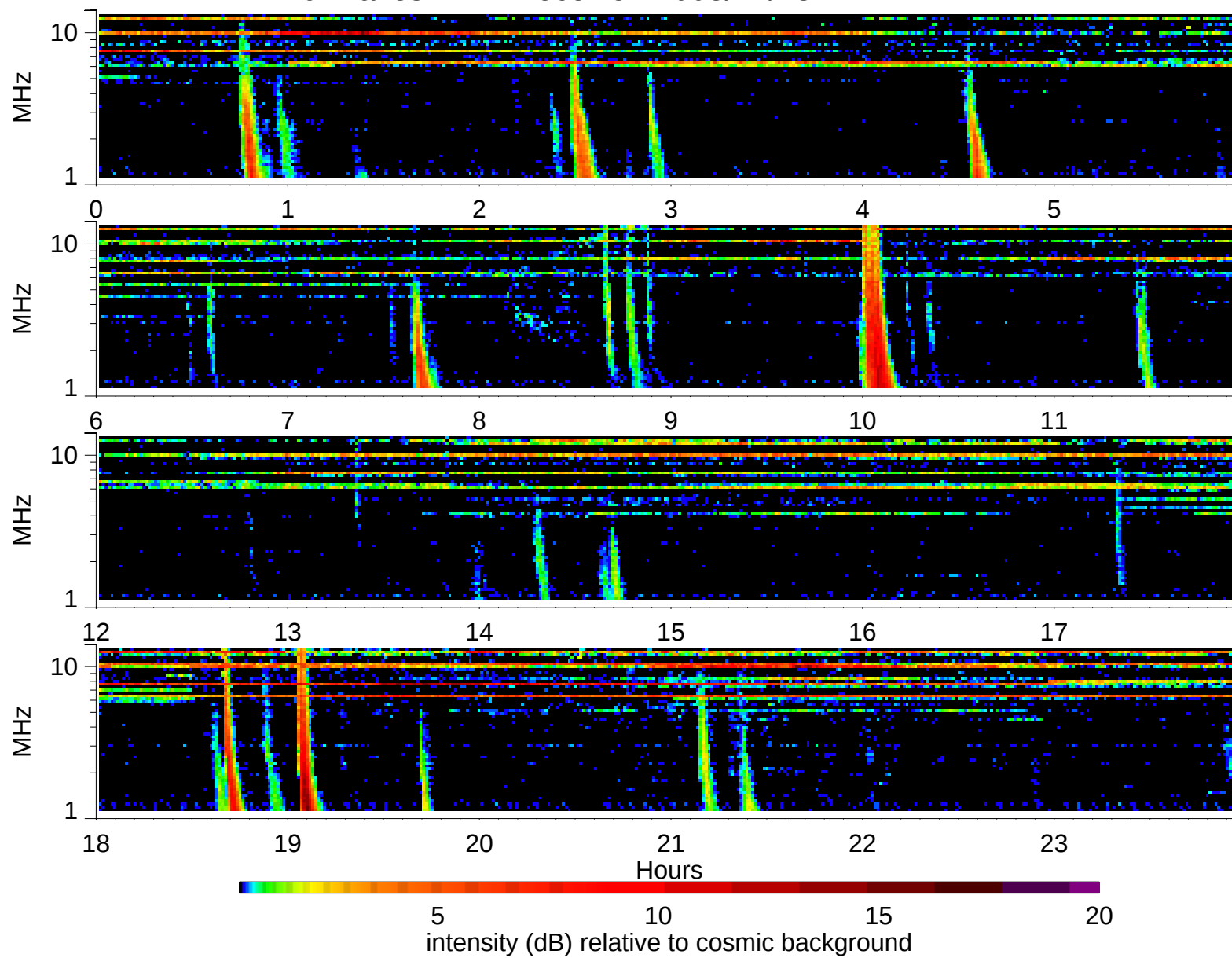
Wind Waves RAD2 receiver: 2003/11/23
