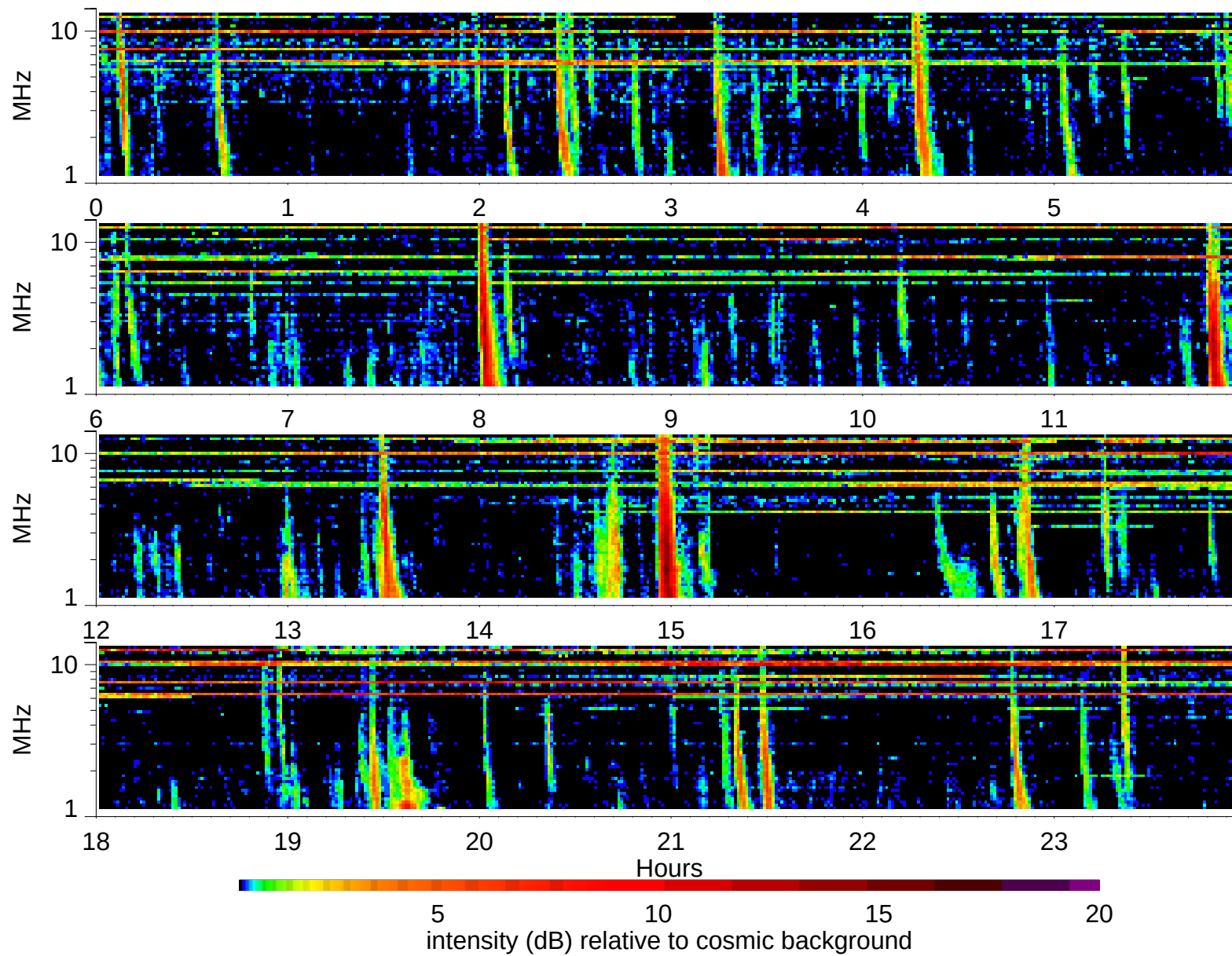
Wind Waves RAD2 receiver: 2003/11/19
