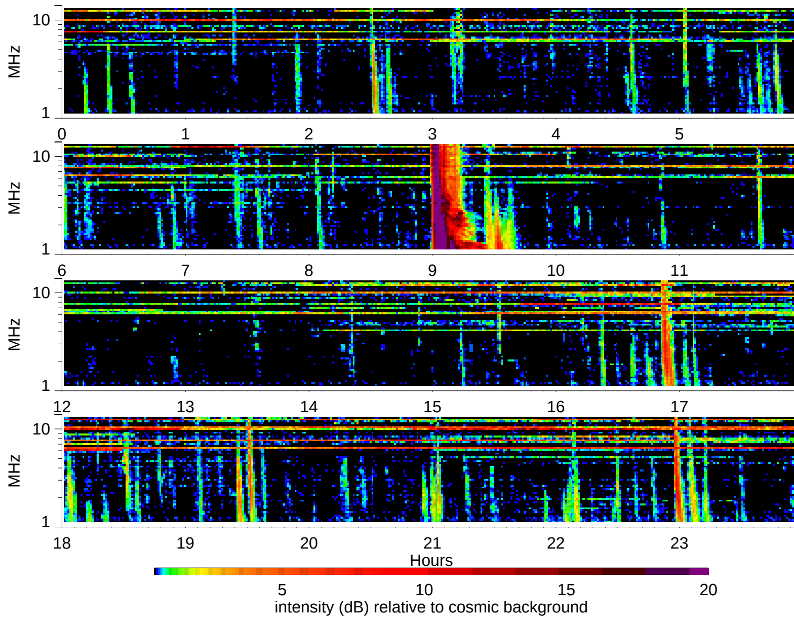
Wind Waves RAD2 receiver: 2003/11/17
