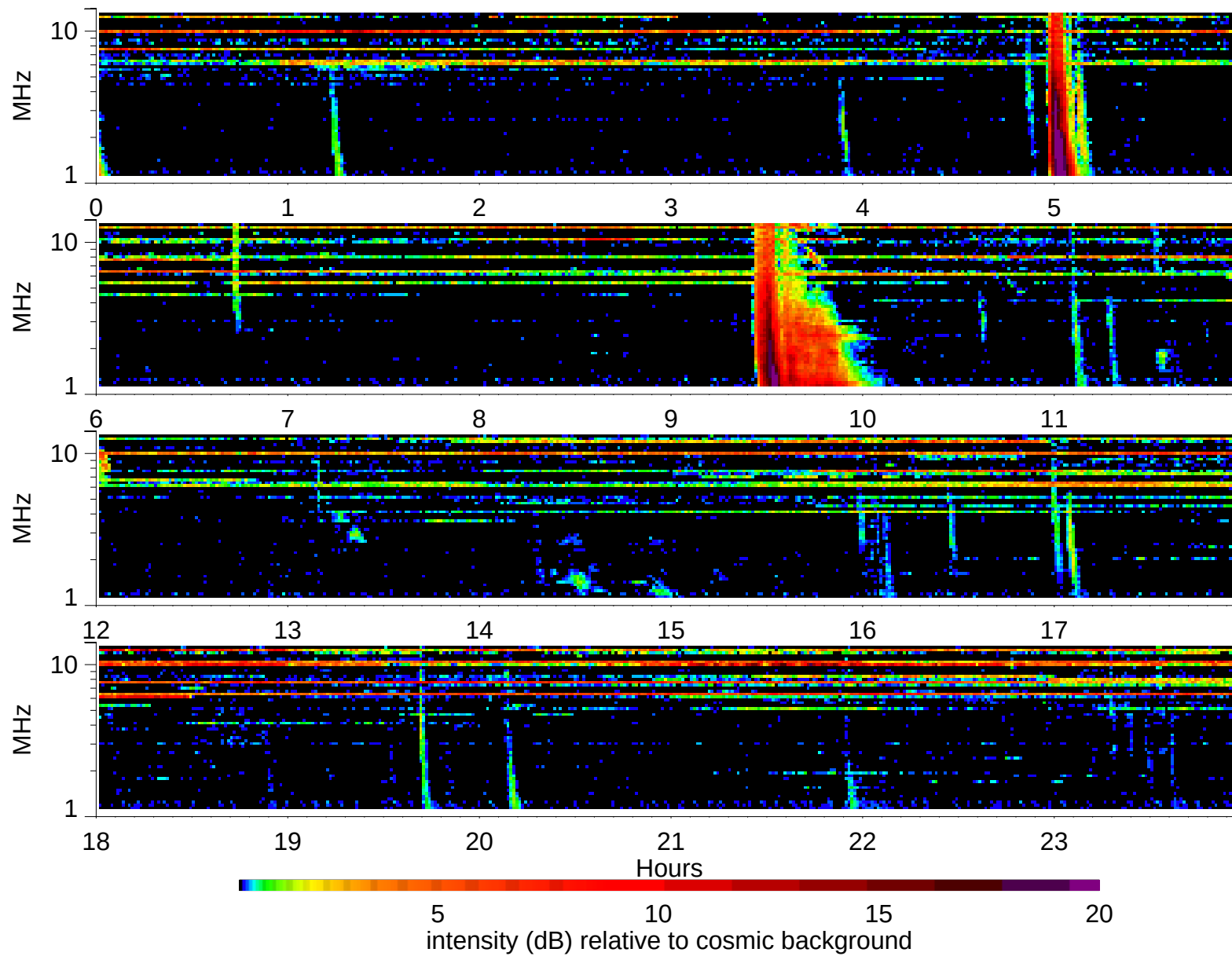
Wind Waves RAD2 receiver: 2003/11/13
