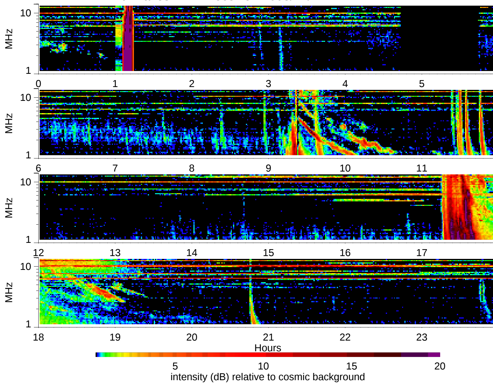
Wind Waves RAD2 receiver: 2003/11/2
