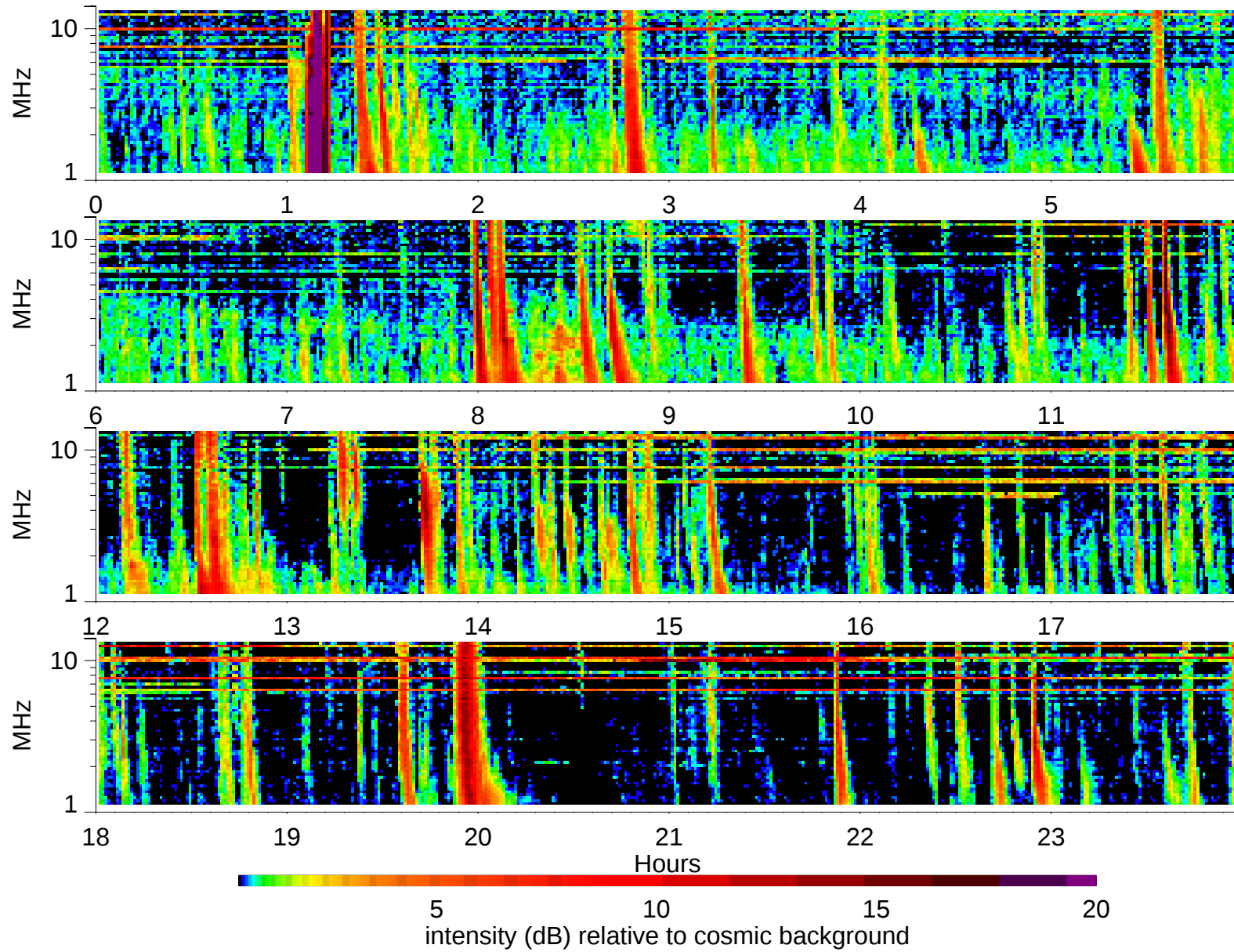
Wind Waves RAD2 receiver: 2003/10/27
