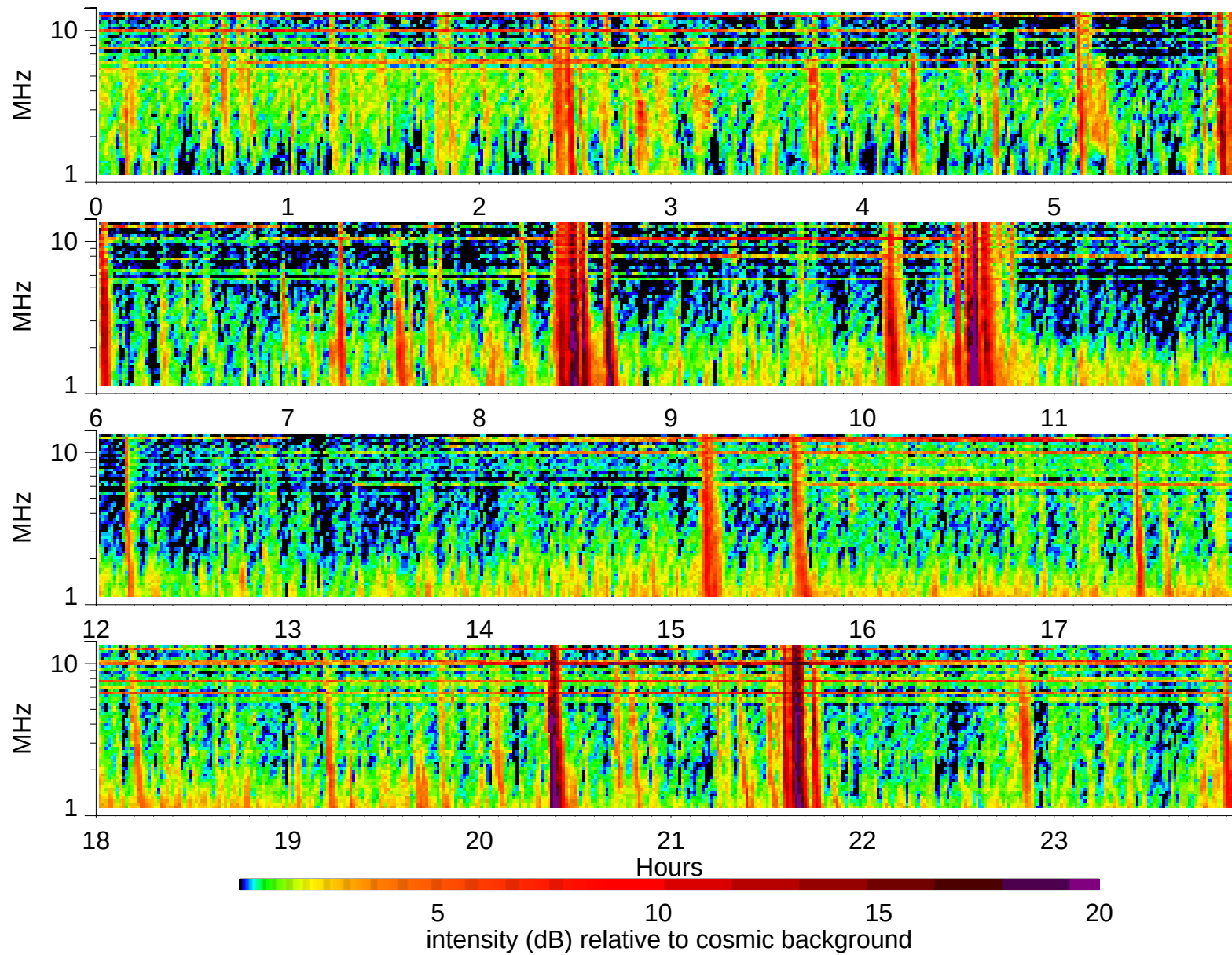
Wind Waves RAD2 receiver: 2003/10/24
