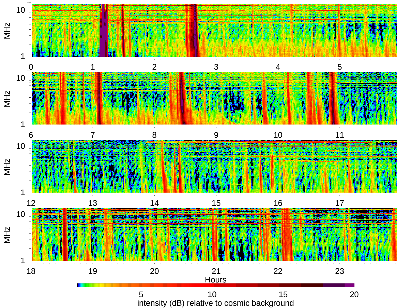
Wind Waves RAD2 receiver: 2003/10/23
