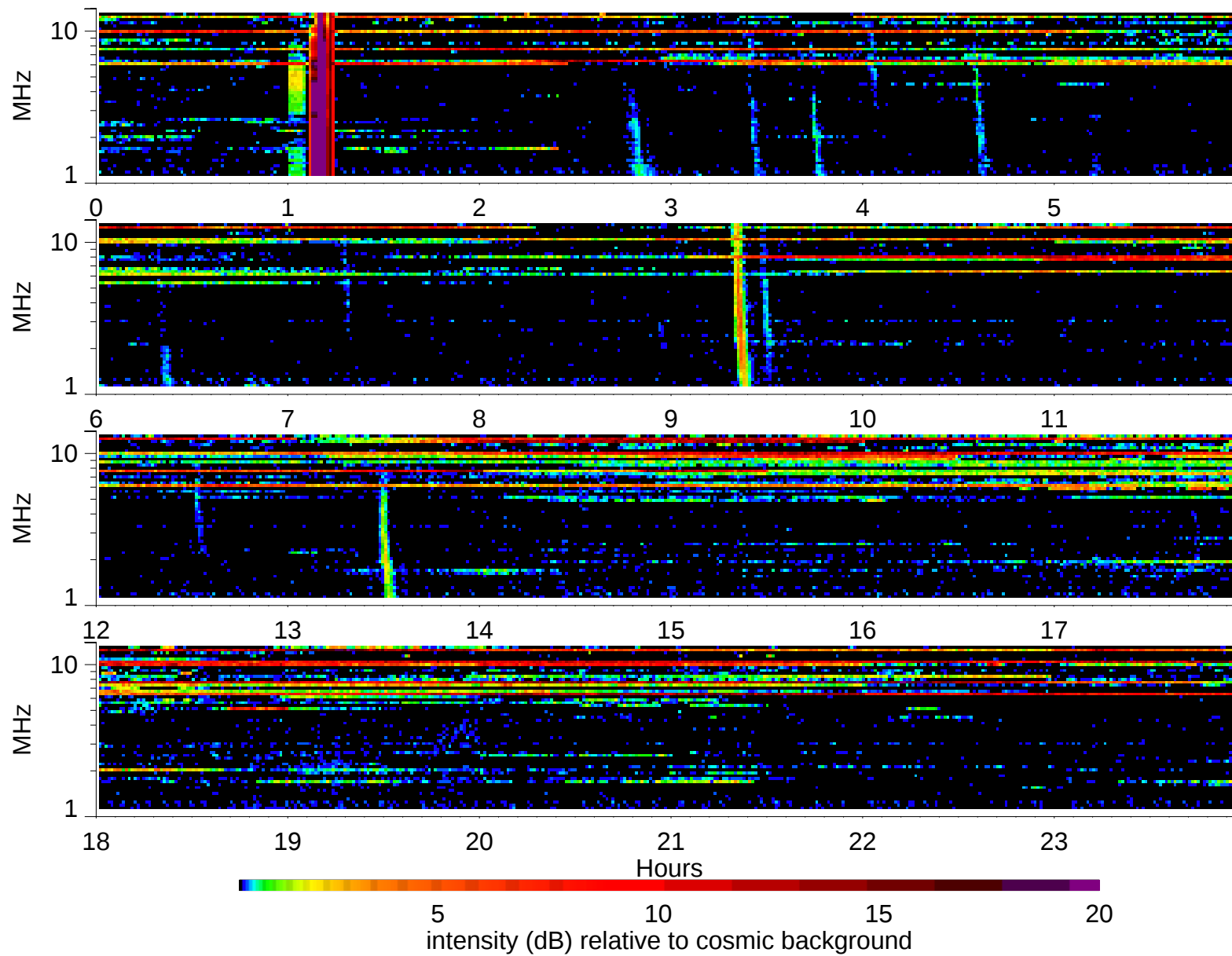
Wind Waves RAD2 receiver: 2003/10/15
