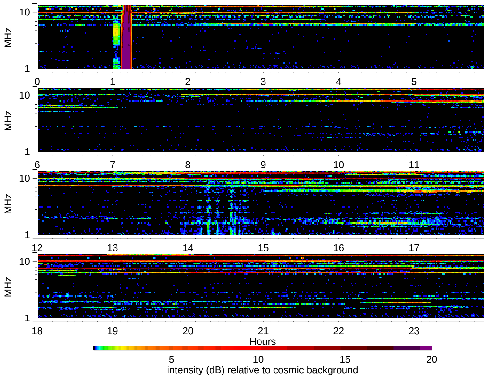
Wind Waves RAD2 receiver: 2003/10/13
