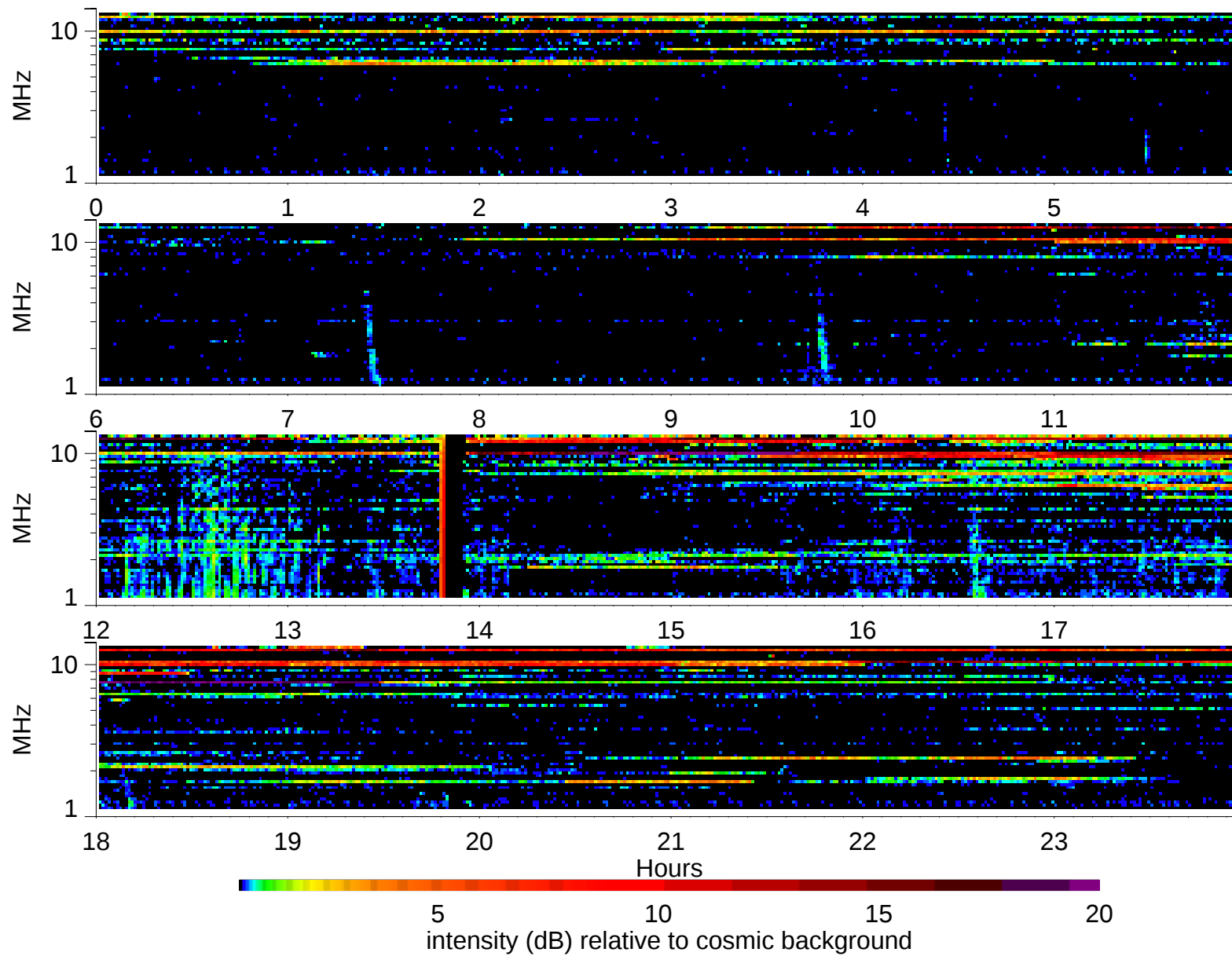
Wind Waves RAD2 receiver: 2003/10/12
