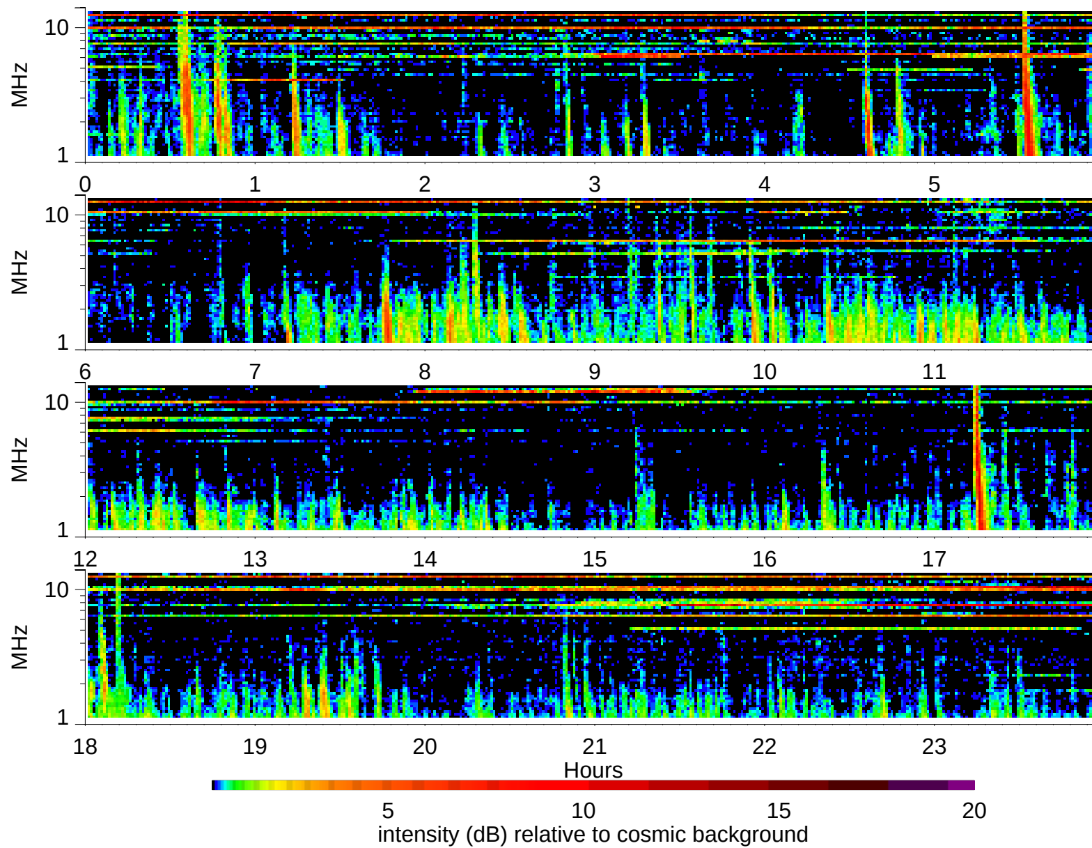
Wind Waves RAD2 receiver: 2003/9/28
