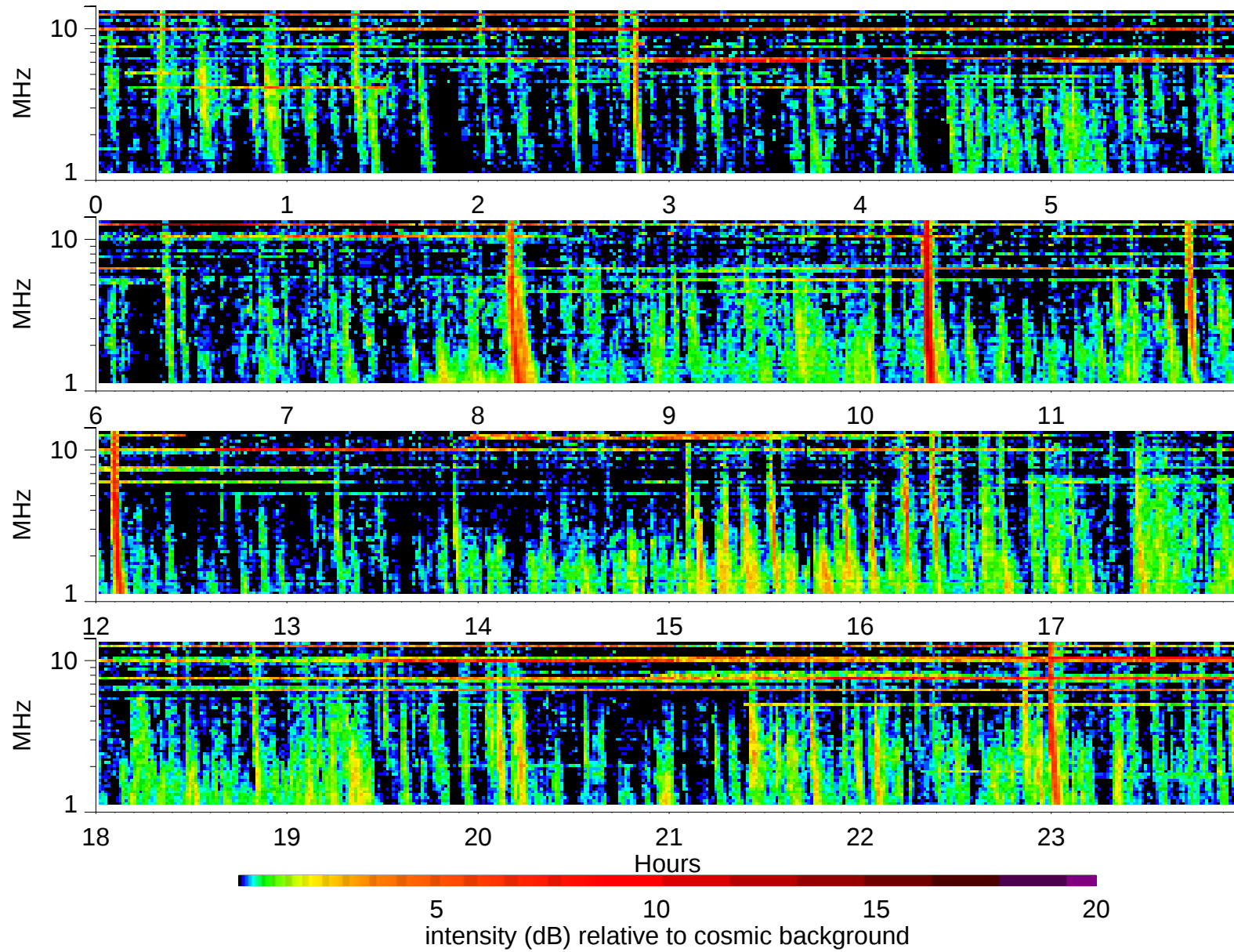
Wind Waves RAD2 receiver: 2003/9/26
