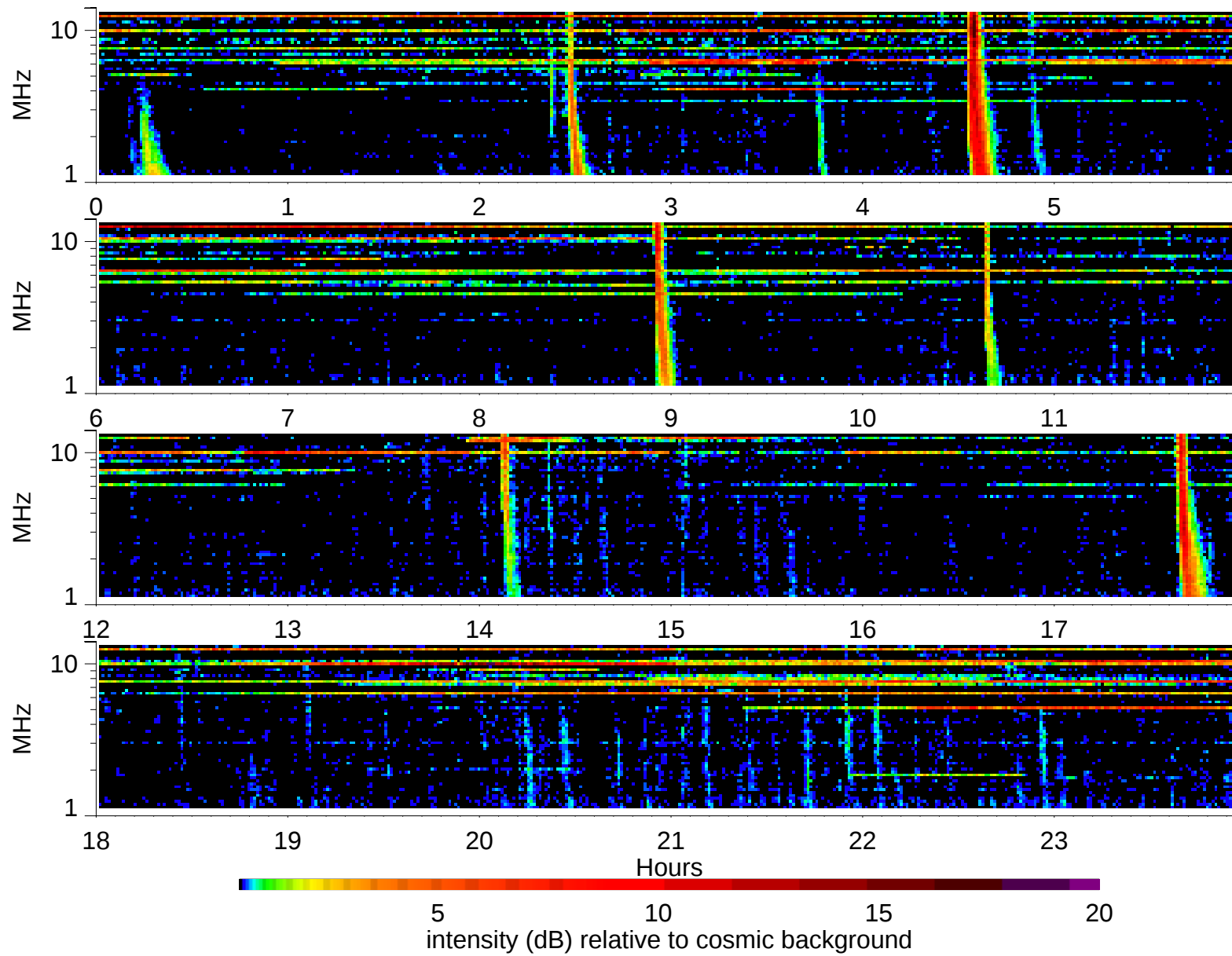
Wind Waves RAD2 receiver: 2003/9/24
