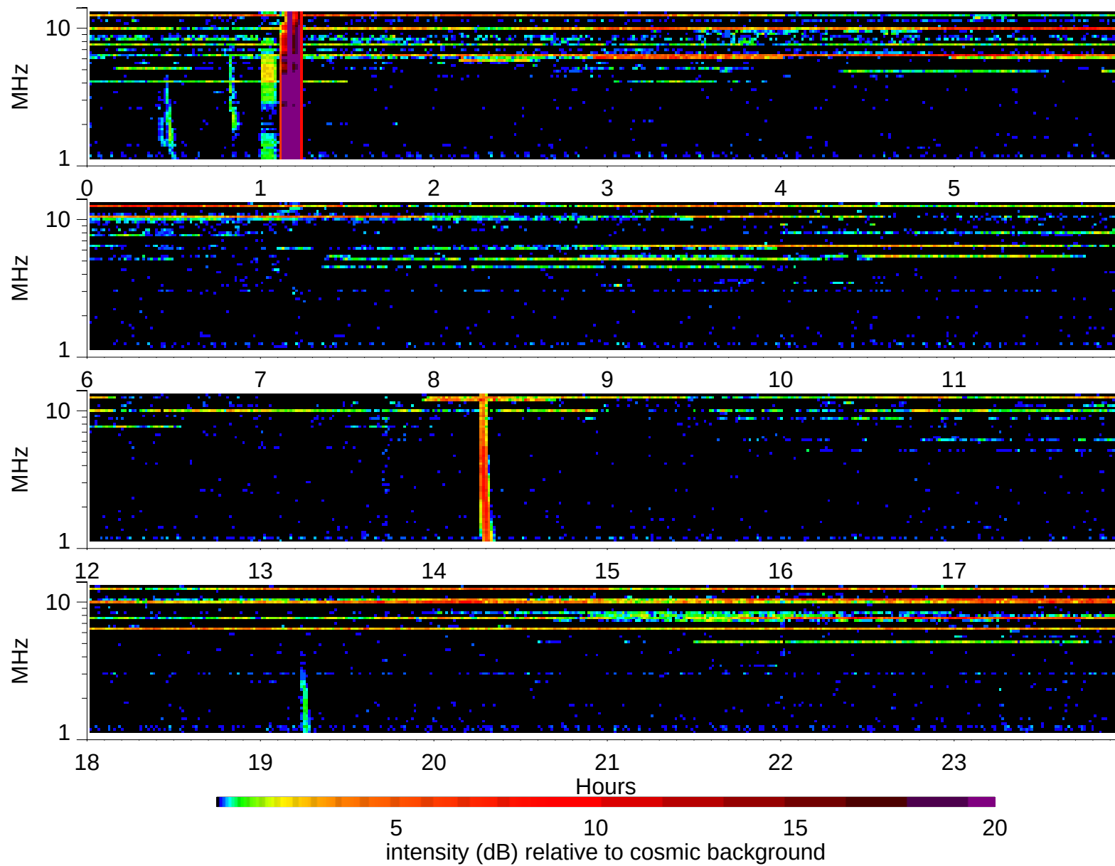
Wind Waves RAD2 receiver: 2003/9/15
