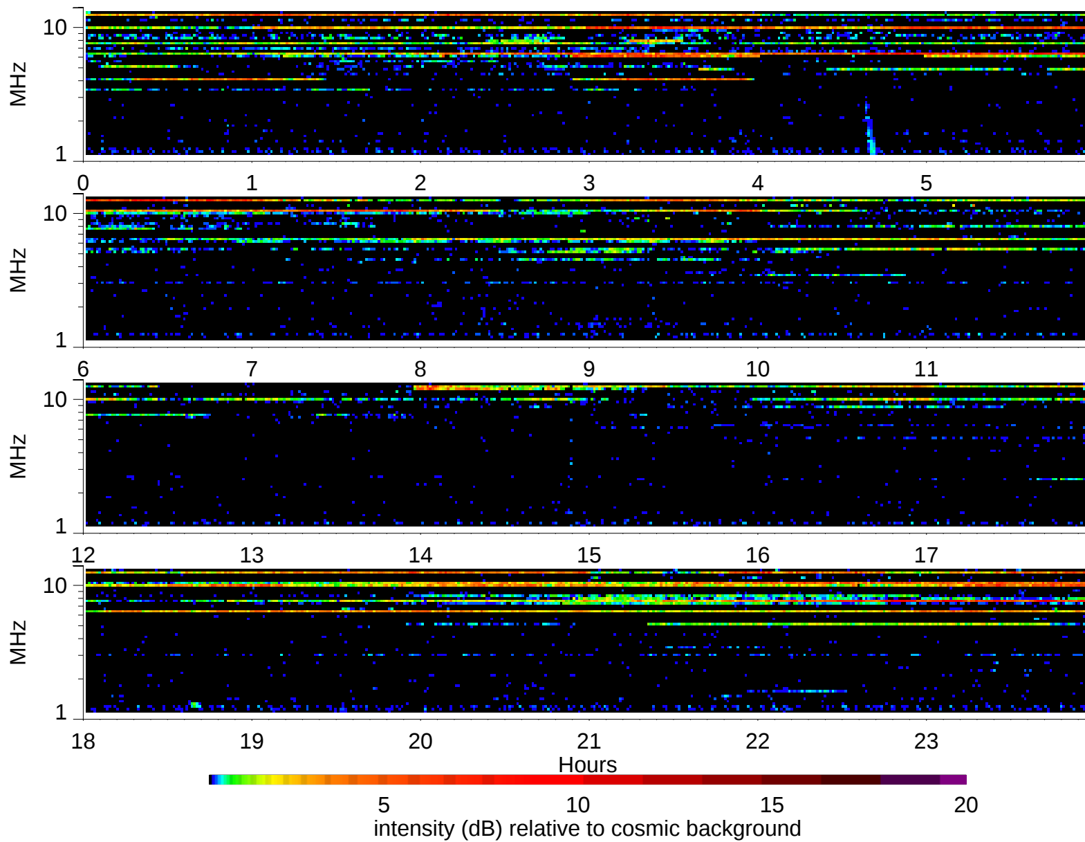
Wind Waves RAD2 receiver: 2003/9/14
