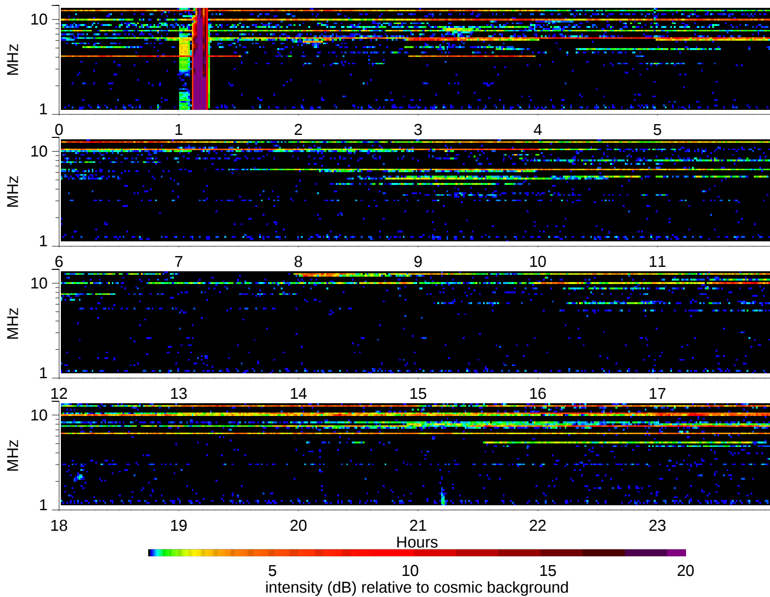
Wind Waves RAD2 receiver: 2003/9/13
