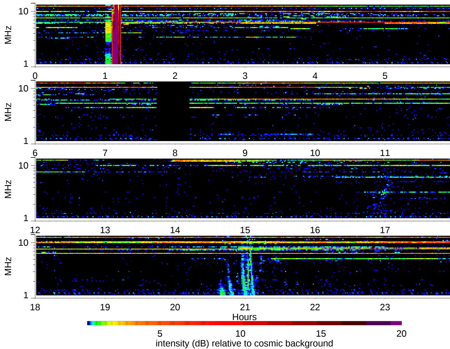
Wind Waves RAD2 receiver: 2003/9/11
