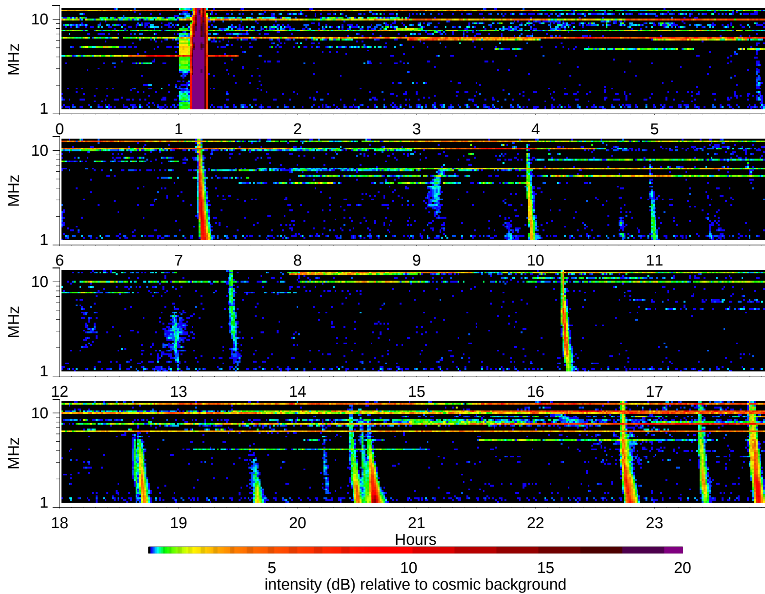
Wind Waves RAD2 receiver: 2003/9/9
