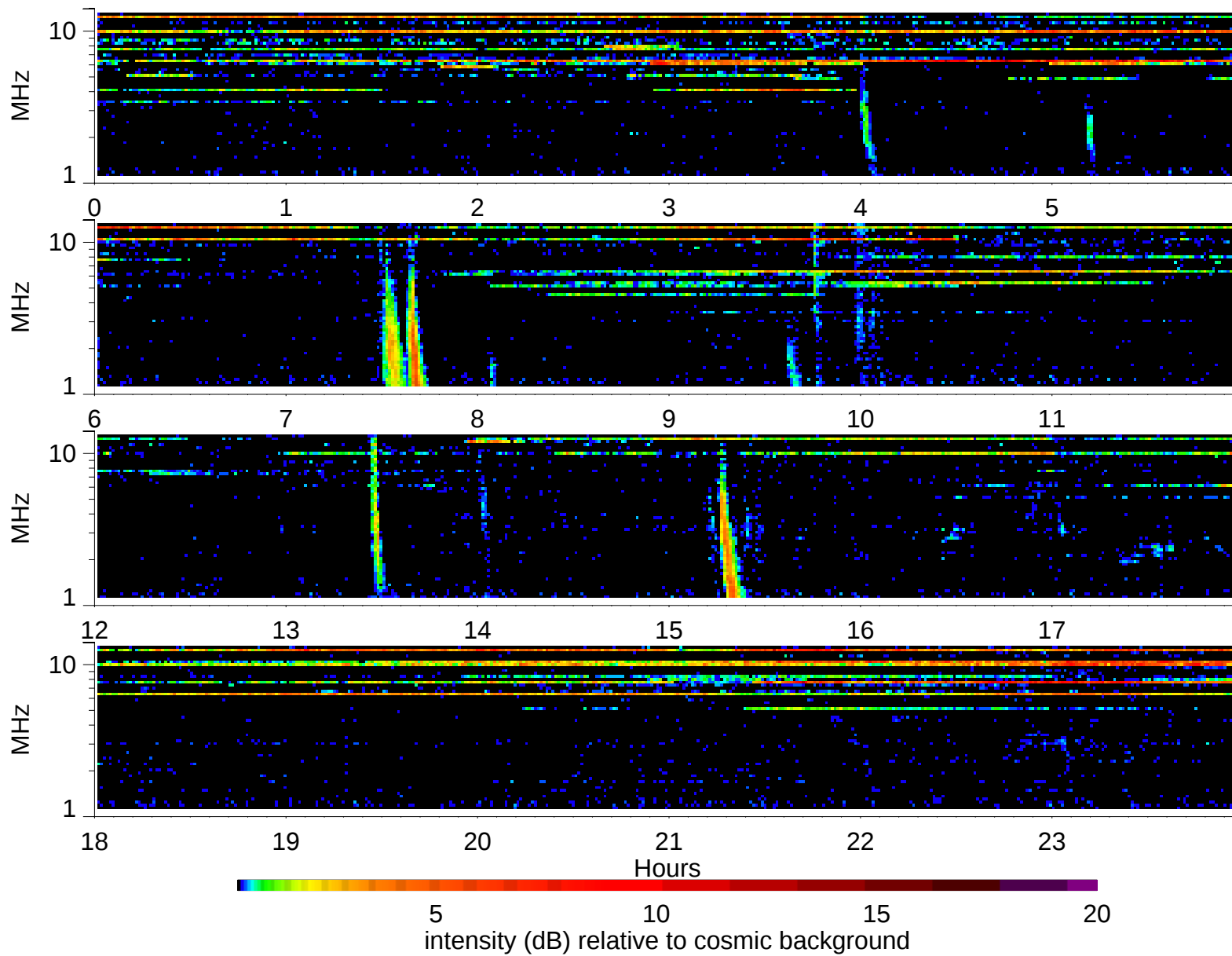
Wind Waves RAD2 receiver: 2003/9/8
