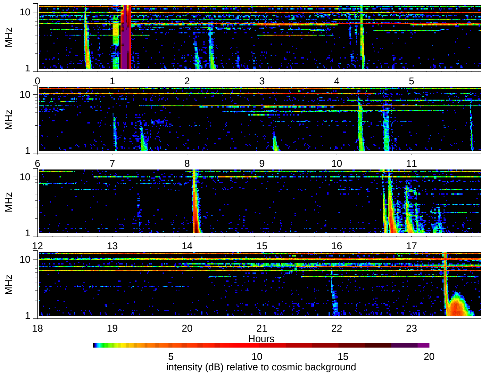
Wind Waves RAD2 receiver: 2003/9/7
