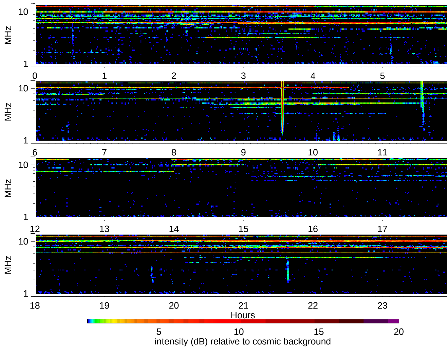
Wind Waves RAD2 receiver: 2003/8/31
