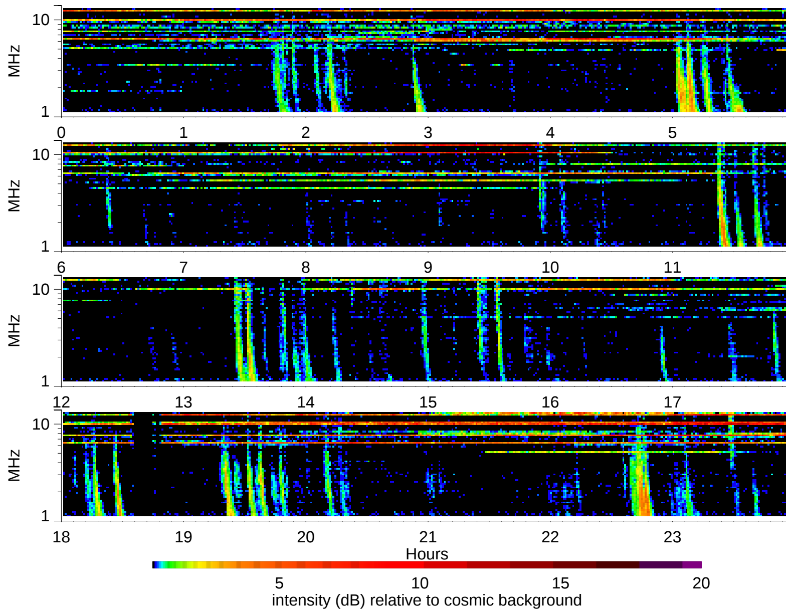
Wind Waves RAD2 receiver: 2003/8/27
