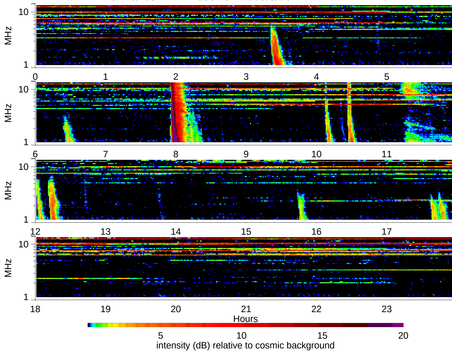
Wind Waves RAD2 receiver: 2003/8/19
